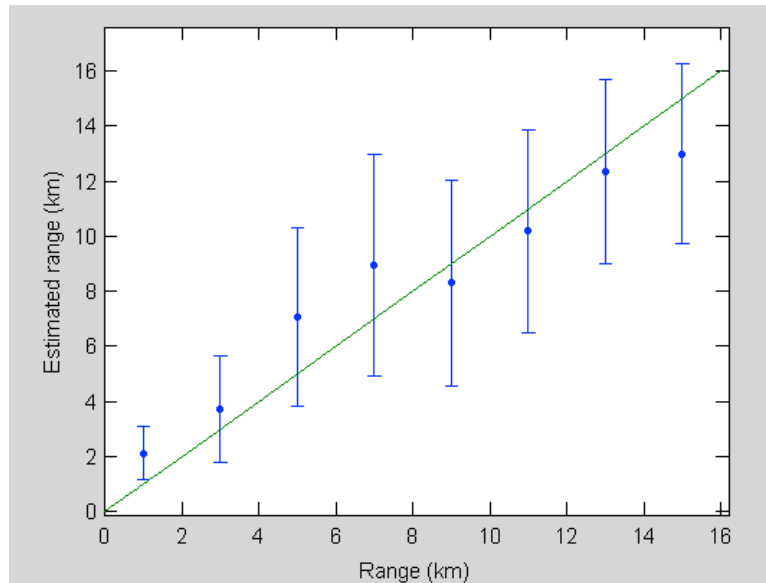
Figure 3. Estimated range vs. tracked range at the Endeavour segment location. Each blue point shows the mean range within that 2km range bin, with error bars indicating standard deviation.
