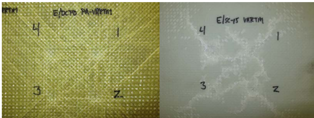
Fig. 18 Front-face damage for composites (left) PPG E-glass-p-DCPD and (right) PPG E-glass-SC-15
