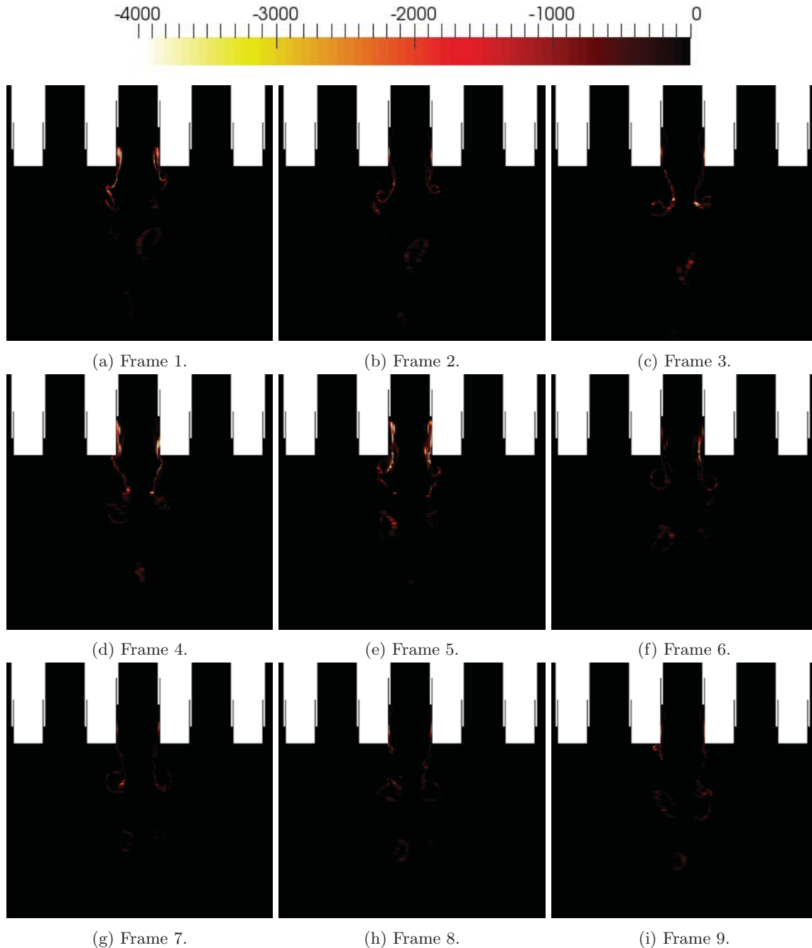
Figure 14: Consumption of C_2H_6 near the study element in the center of the combustor. Frame numbers correspond to the points identified in Figure 8.
