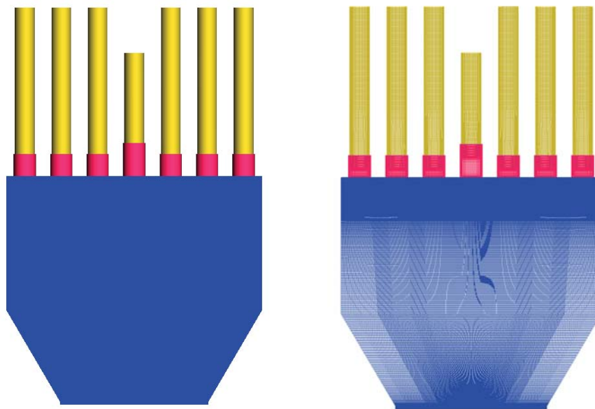
Figure 2: Model geometry (left) showing oxidizer tubes (in yellow) and fuel tubes (in Red). The computational Mesh is shown to the right and contains 15.63 million hexahedral cells.
