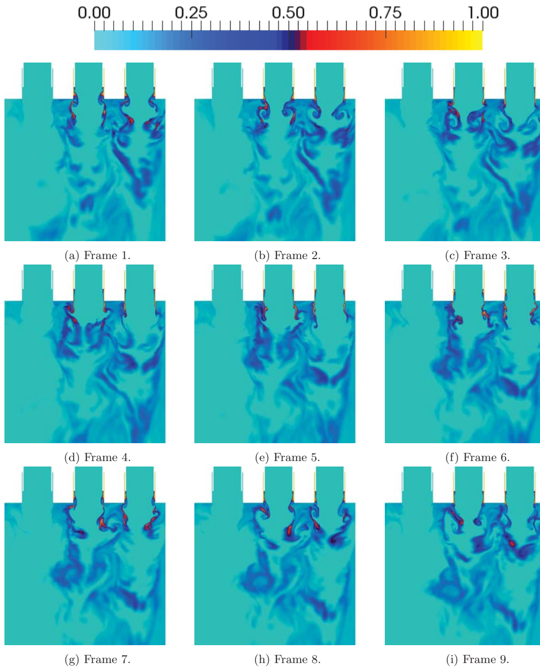
Figure 11: Mass fraction of RP1 near driving elements on the right side of the combustor. Frame numbers correspond to the points identified in Figure 8.
