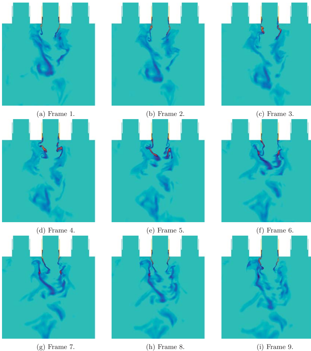
Figure 18: Mass fraction of RP1 near driving elements on the right side of the combustor. Frame numbers correspond to the points identified in Figure 16.
