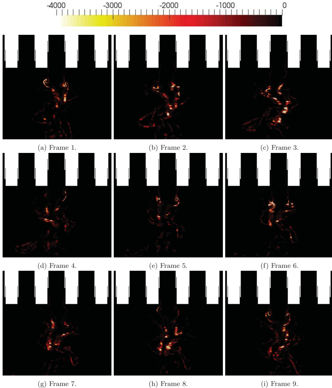
Figure 21: Consumption of C_2H_6 near the study element in the center of the combustor. Frame numbers correspond to the points identified in Figure 16.
