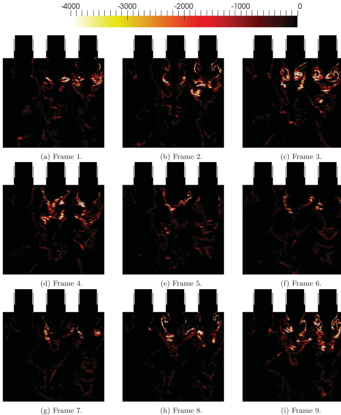
Figure 12: Consumption of RP1 near driving elements on the right side of the combustor. Frame numbers correspond to the points identified in Figure 8.
