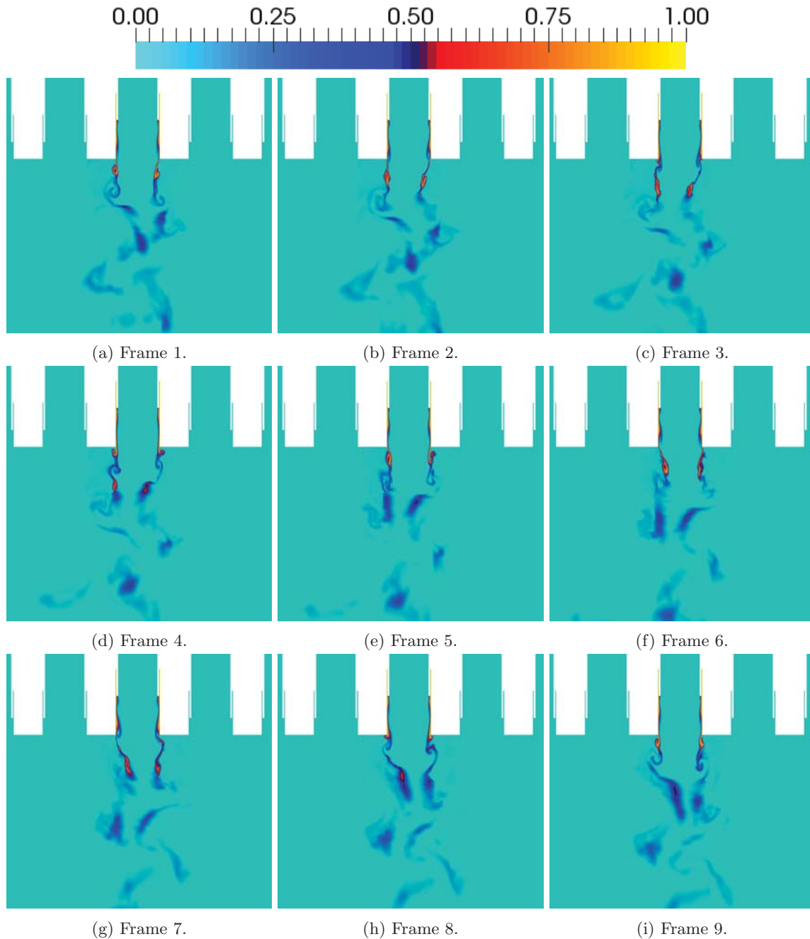
Figure 20: Mass fraction of C_2H_6 near the study element in the center of the combustor. Frame numbers correspond to the points identified in Figure 16.
