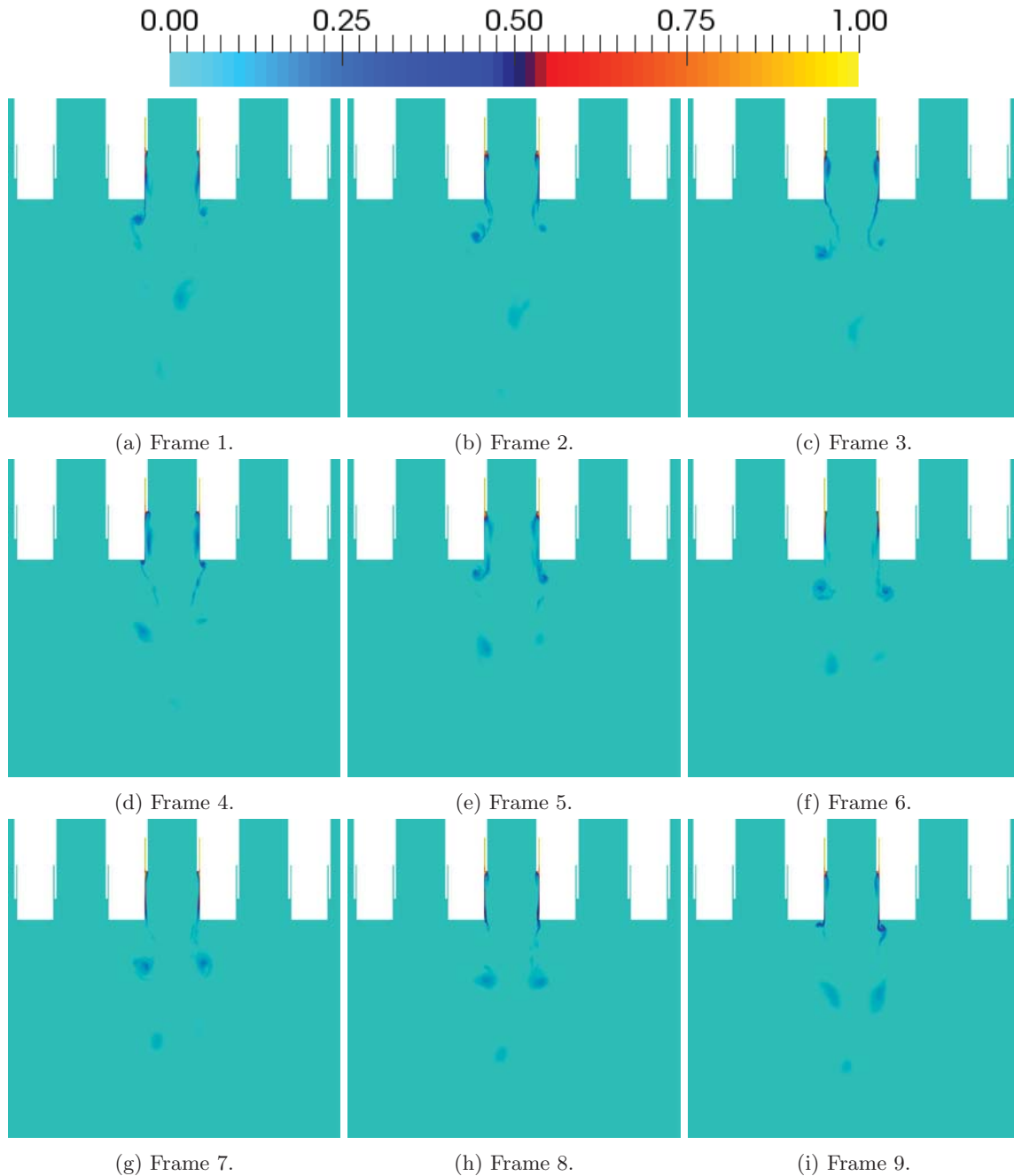
Figure 13: Mass fraction of C_2H_6 near the study element in the center of the combustor. Frame numbers correspond to the points identified in Figure 8.
