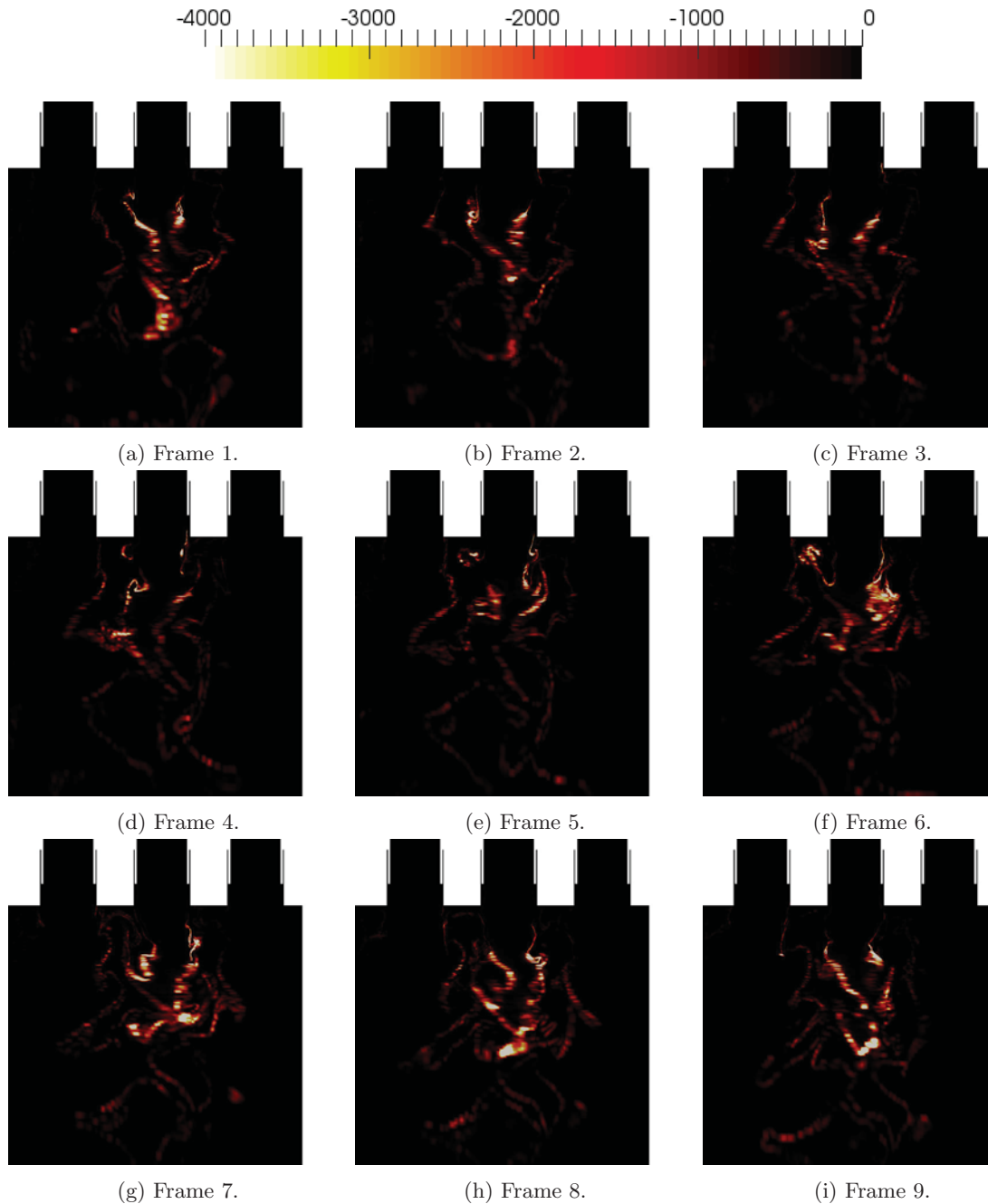
Figure 19: Consumption of RP1 near driving elements on the right side of the combustor. Frame numbers correspond to the points identified in Figure 16.
