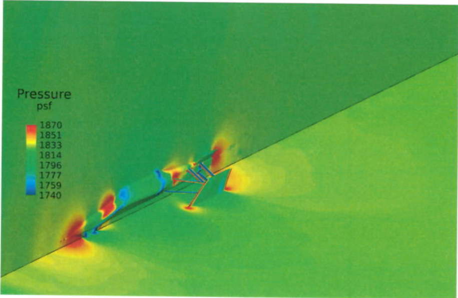
Pressure Distribution Mach 0.5
