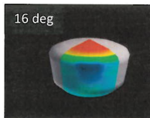
Maraia Capsule Pressure Contours 14, 16, 18 degrees ( M=0.45 )
