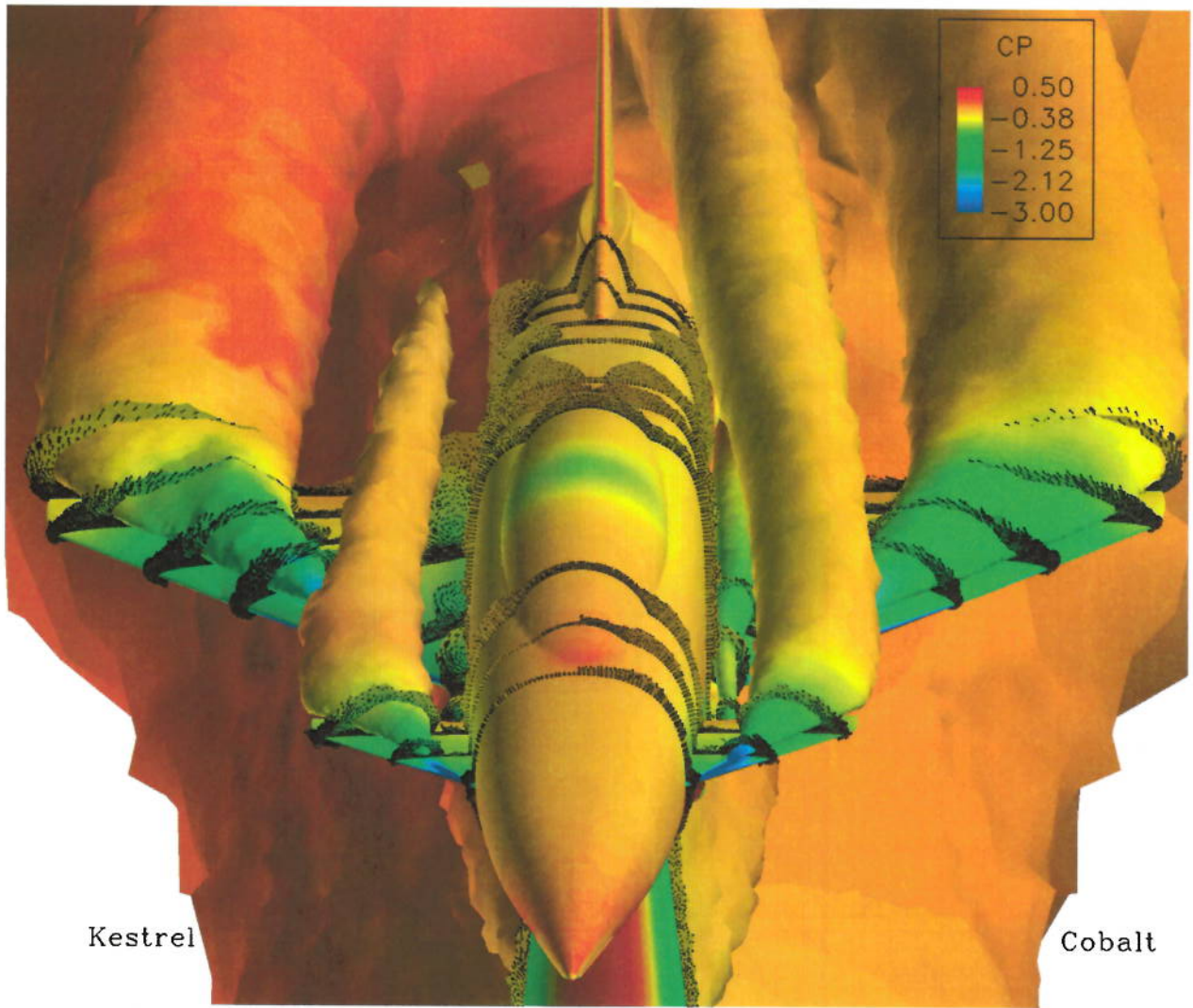
X-31 predicted vertical flows of Cobalt and Kestrel solvers
