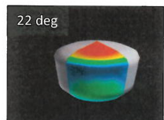
Maraia Capsule Pressure Contours 18, 20, 22 degrees ( M=0.45 )
