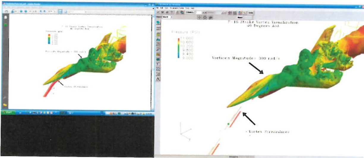
Vortex visualization
