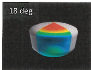
Maraia Capsule Pressure Contours 18, 20, 22 degrees ( M=0.45 )
