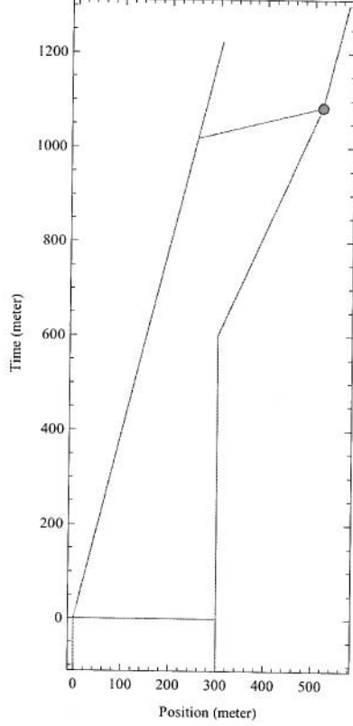
Figure 2: Space-time path for two clocks connected by a stiff rod. The left side of the rod receives an impulse at t = 0 and begins to move with a velocity v . The right side of the rod does not begin to move until the signal reaches it at the speed of sound v_s . At the time the sound wave reaches the far end, it begins to move with a recovery speed v_r until the rod reaches a new equilibrium length L + \Delta L .
