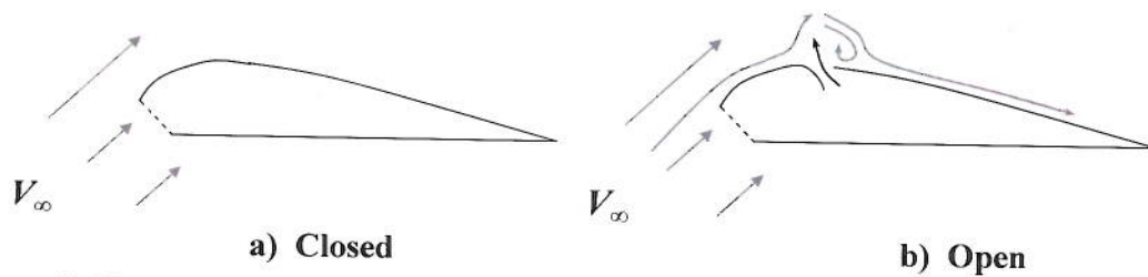
Figure 1. Notional depiction of parafoil aerodynamics with upper surface bleed air spoiler 5
