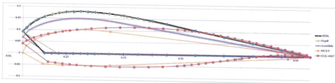
Figure 2. Ram-air airfoil sections
