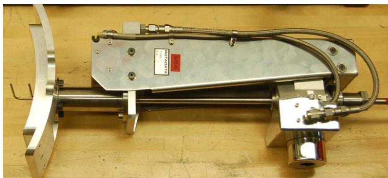
Figure 7. 5-Hole probe rake installed in traverse and mounted to AIP window plug.
