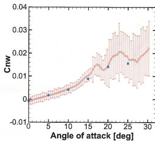
(f) Yaw moment coefficient
