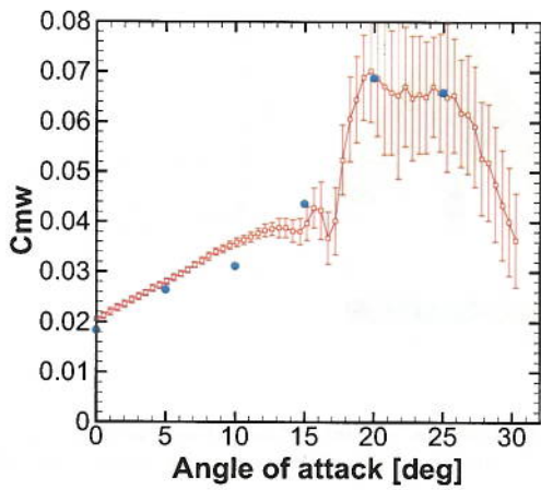
(e) Pitch moment coefficient
