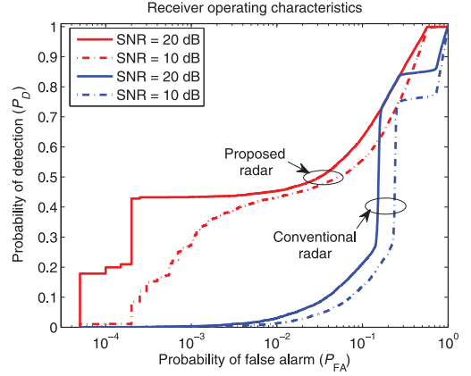
Fig. 2. Improved detection performance using the proposed radar.
