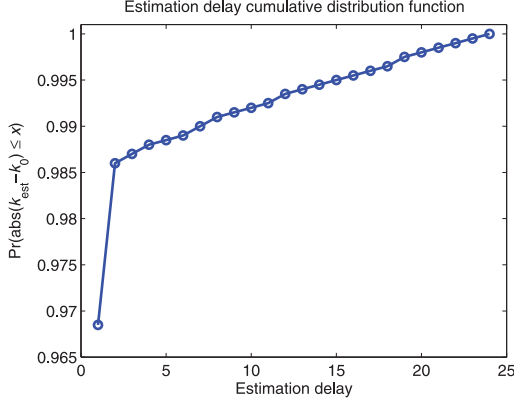
Fig. 1. Performance of the change point detection test in terms of the cumulative distribution function of the estimation delay.
