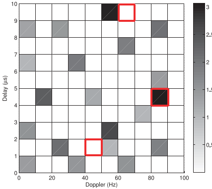
Fig. 5. Target estimates at SNR of -21.58 dB by designing only B .
