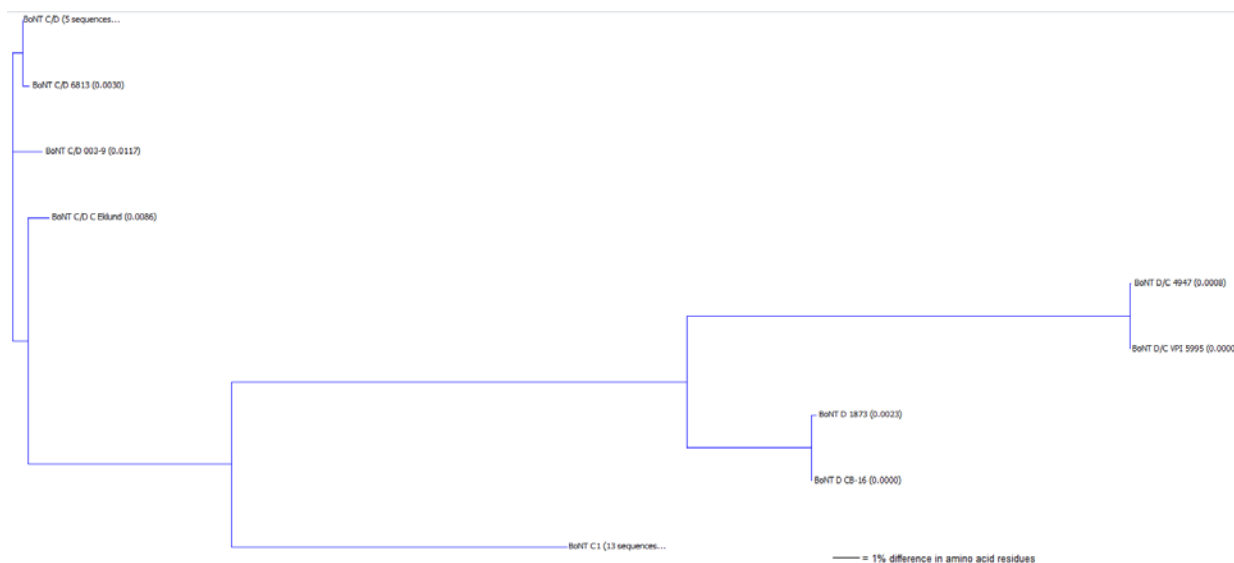
Figure 4. Dendrogram showing the relationships of BoNT/C and /D subtypes. A total of 23 amino acid sequences were analyzed. The mosaic nature of the BoNT/C and /D subtypes results in large differences in amino acid sequence (23.5-48.8%).
