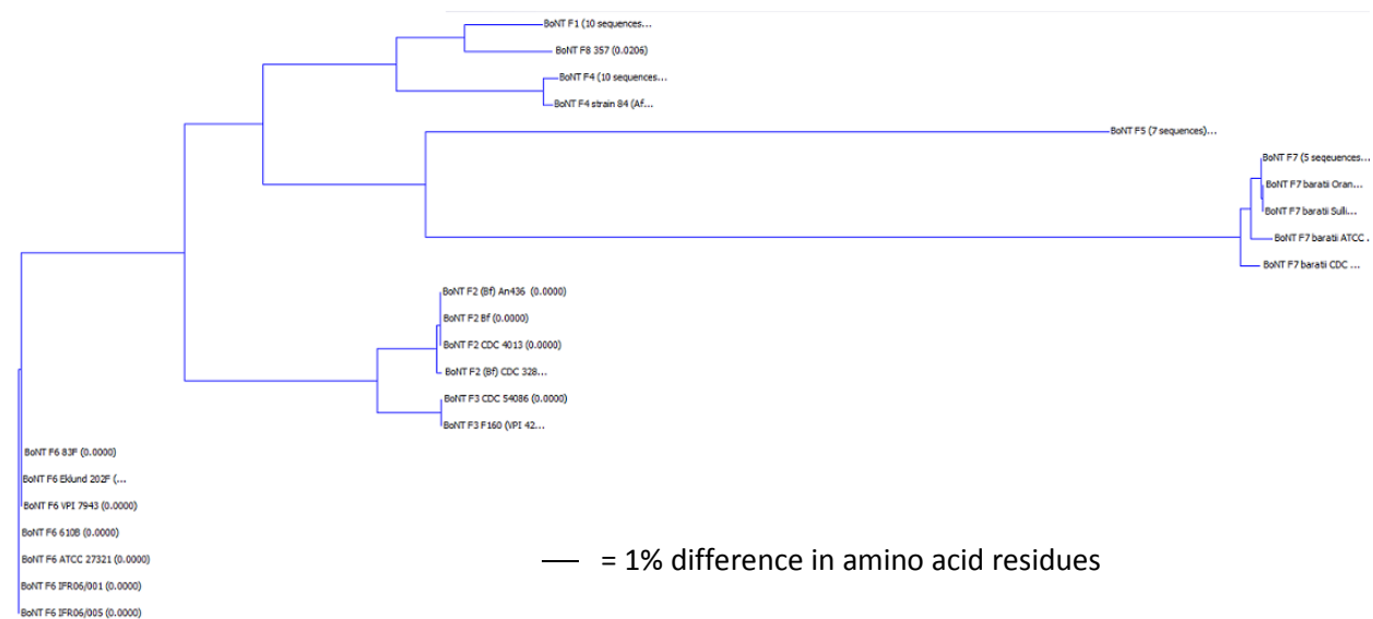
Figure 6. Dendrogram showing the relationships of BoNT/F subtypes. A total of 52 amino acid sequences were analyzed. The scale for this dendrogram is significantly smaller than with the others due to the wider range of identity differences (7.8-36.2%) within this serotype.
