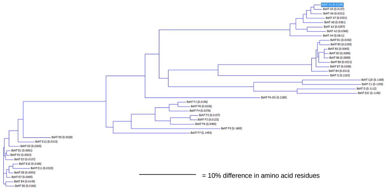
Figure 1. Dendrogram showing the relationship of all published/publicly posted BoNT subtypes. The dendrograms were generated using ClustalW using representatives listed in Table 3. BoNT/FA (H) is also known as BoNT/HA.
