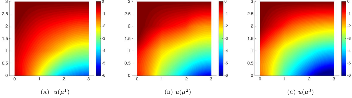
FIGURE 5. Thermal block synthetic problem: example of the true field for three values of the parameters.
