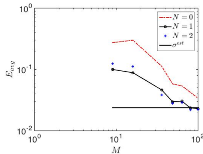
FIGURE 9. Thermal patch problem: convergence with M for fixed N .
