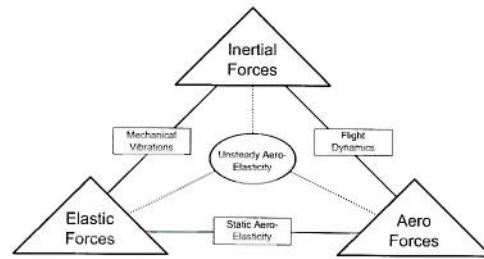
Figure 1. Modified Collar's triangle representing the forces at play in an aeroelastic system.
