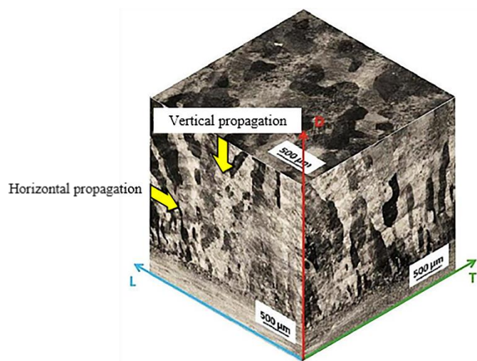
Fig. 12. 3D illustration of horizontal and vertical fatigue crack propagation.
