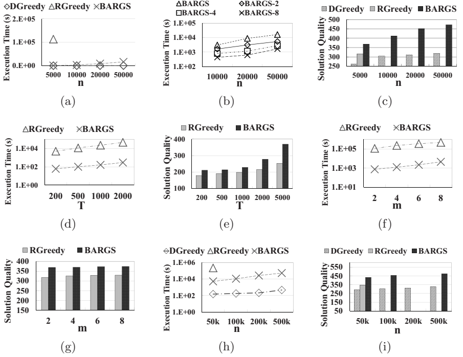
Fig. 2. Experimental results on Facebook and DBLP datasets
