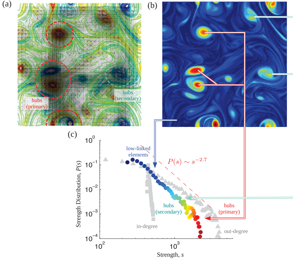
Figure 8.2: The scale-free network of vortical interactions in two-dimensional turbulence with initial Re(t_0) = 814 . (a) Turbulent network structure overlaid on the vorticity field with the darkness of the network edges corresponding to the values of the adjacency weights ( t = 18 ). (b) Contour plot of the node strength s distribution. Vortex cores having high degree of connectivity act as hubs in the turbulent vortical network. (c) The corresponding node strength probability distribution exhibiting the scale-free characteristics with P \sim s^{-2.7} . The same contour level is shared by (b) and (c). Also shown in the background of (c) in gray are the out and in-degree distributions ( \phi = 0 and 1 , respectively). The network visualized in (a) does not show interactions from periodic images and uses 32 \times 32 nodes for graphical clarity.
