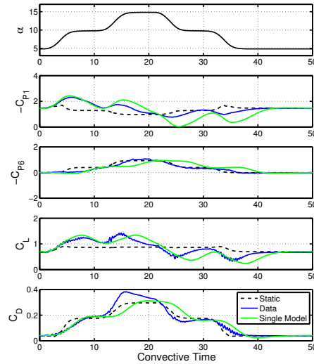
Figure 3.7: Performance of a single ( 5 – 10^\circ pitch-up) model in predicting pressure and force coefficients for double pitch up/down maneuver.
