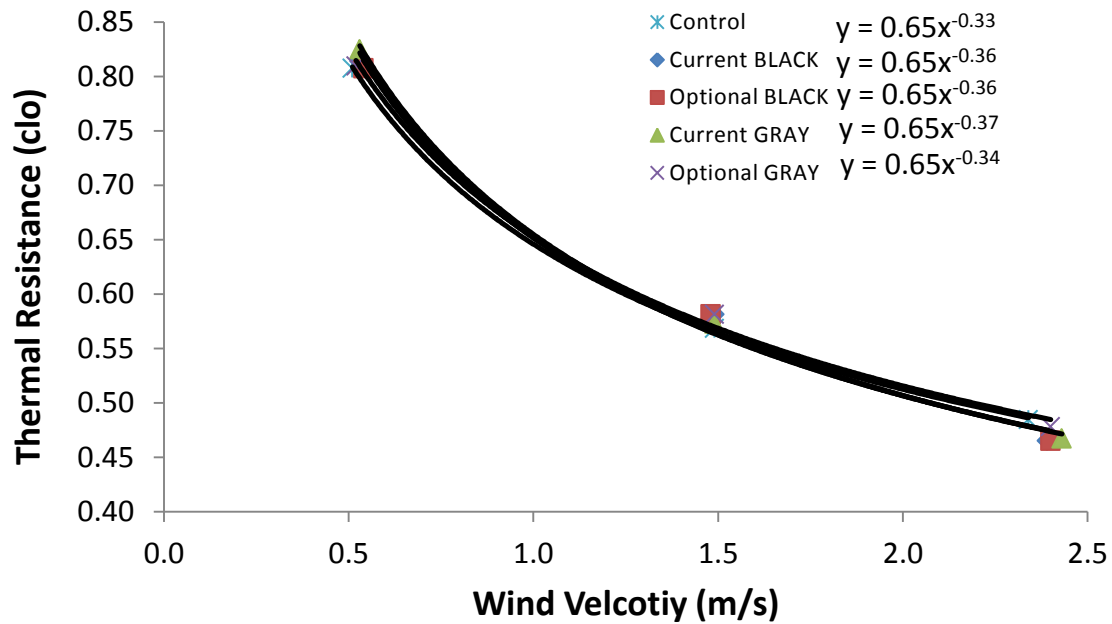
Figure 3. Thermal resistance (clo) for the 5 ensemble configurations
