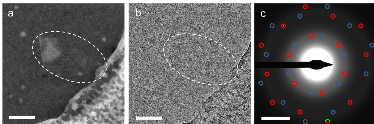
Fig. 9. (a) MAADF-STEM, (b) BF-TEM images and (c) the corresponding diffraction pattern of a graphene flake in a PIM-1 composite membrane showing the flakes are misoriented, suggesting the re-stacking of the flakes. The dash line ellipse in (a–b) indicates the position of the flake. Scale in (a–b) and (c) are 100 nm and 5 nm −1 , respectively. (A colour version of this figure can be viewed online.)
