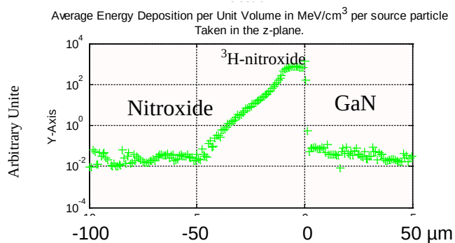
Fig. 7 Energy deposition profile as a function of layer thickness. In this profile, the 3 H-nitroxide is 10 \mu\text{m} , GaN is 100 \mu\text{m} , and nitroxide is 100 \mu\text{m} thick. 3 H-nitroxide is surrounded on both sides to confirm conservation of energy.
