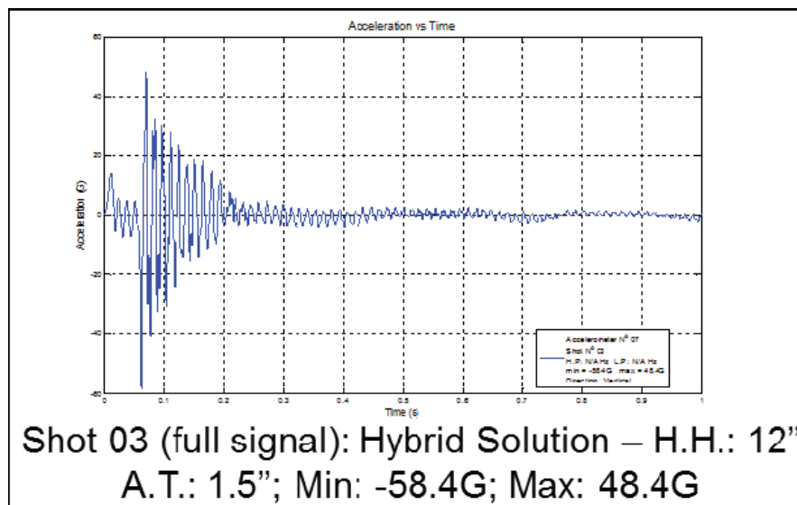
Figure 8 - Acceleration/Time Plot for 1.5" Anvil Travel
