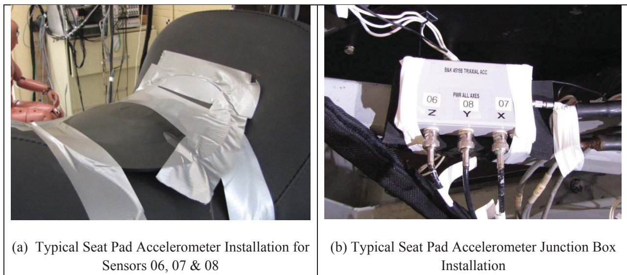
Figure 5 – Typical Seat Pad Accelerometers Installation
