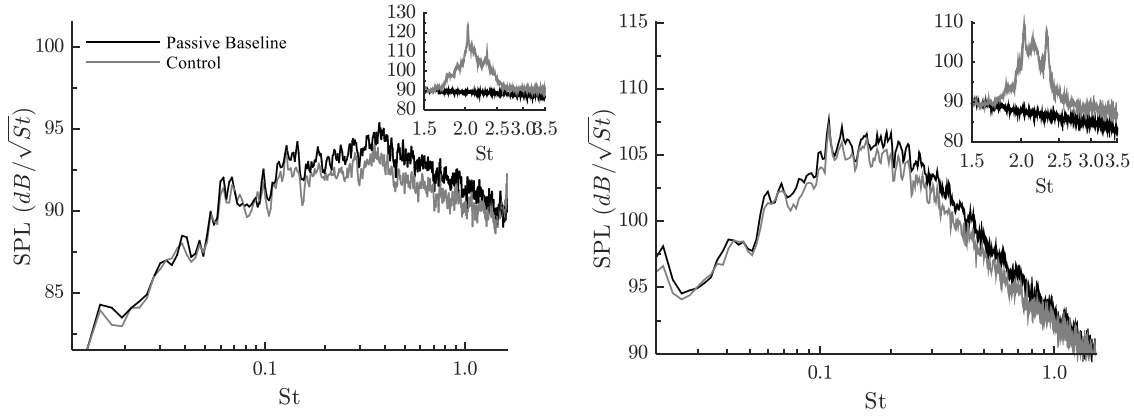
Fig. 7: Acoustic spectra for Mach 0.9 jet (NPR = 1.69) with and without high-frequency actuation showing (a) 90° (b) 150°. Inset: Increase in high frequency noise due to the actuator. The crossover Strouhal number ( St_D = 1.6 ) coincides with the onset of actuator peak.
