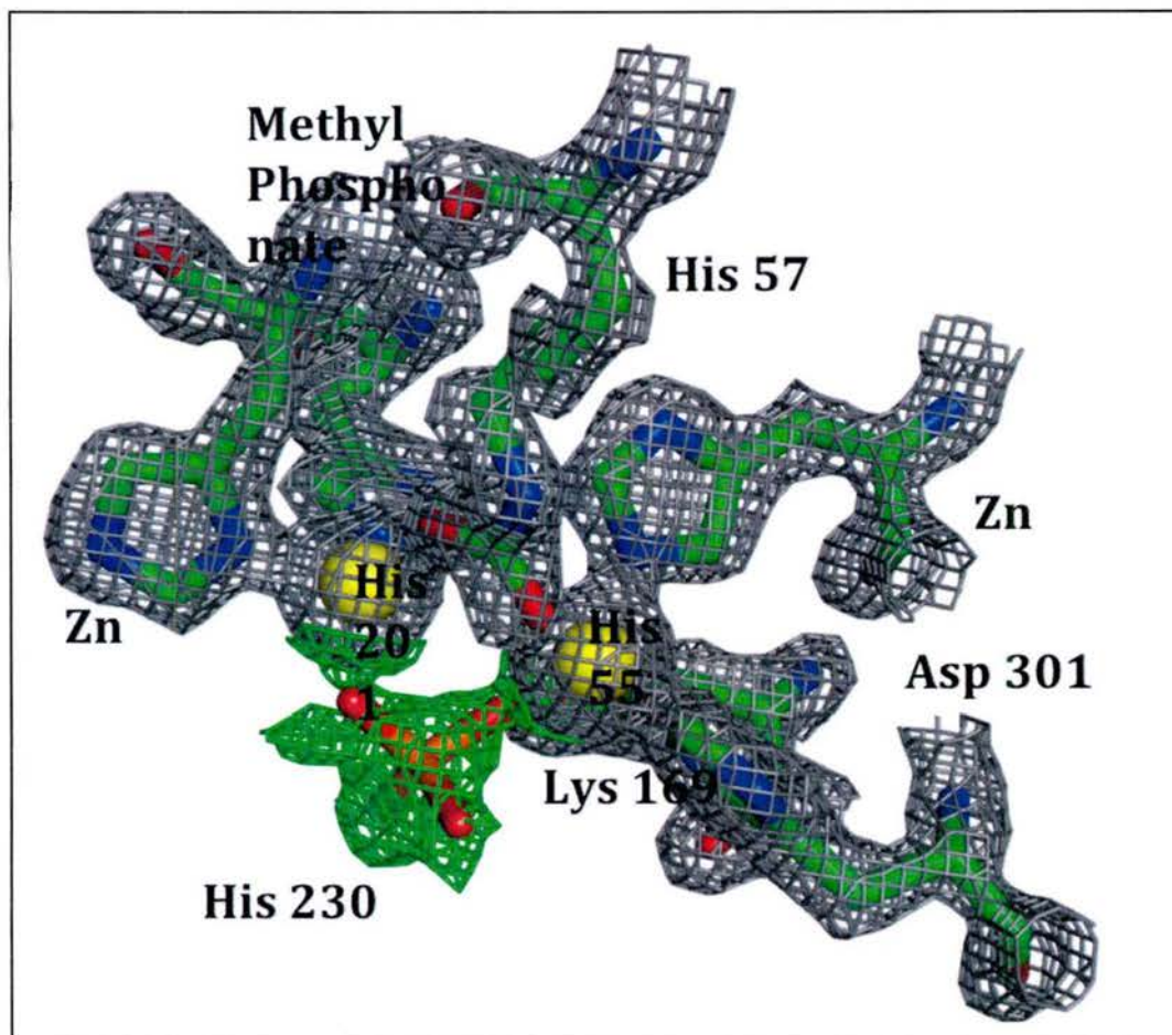
Figure 10: Electron density maps of the active-site region of the PTE_C23_PP structure exhibit electron density (green) corresponding to the methyl phosphonate ( V ). The 2Fo-Fc map contoured at 1 \sigma is shown in gray. The Fo-Fc map contoured at 2.5 \sigma shown in green.
