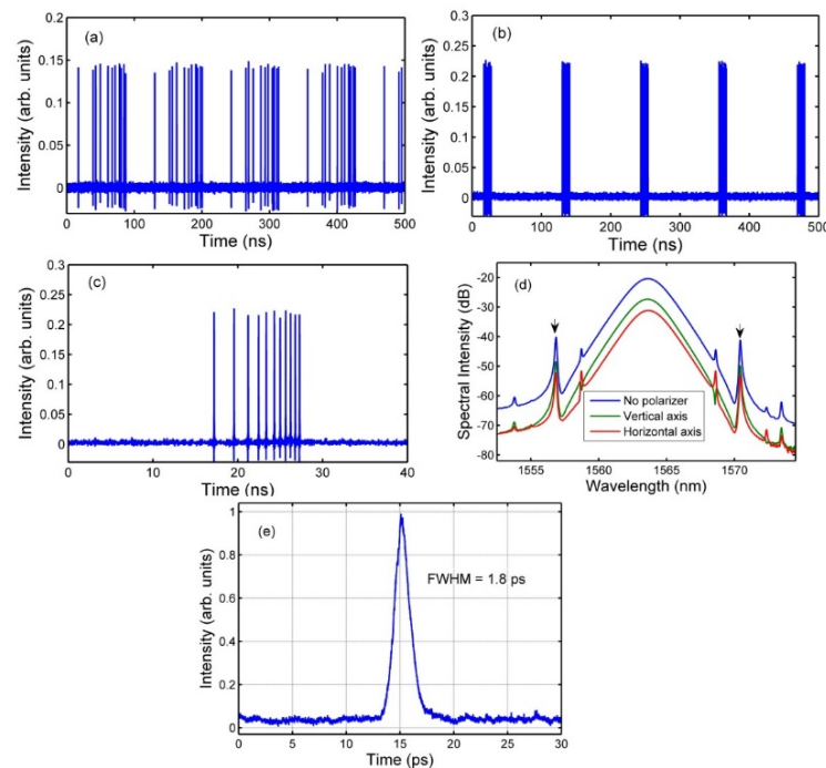
Figure 2.1 Typical bunches of multiple vector solitons formed in the fiber laser. (a) and (b): Two states of the laser emission; (c) The details of the soliton bunch; (d) Polarization resolved optical spectra. Blue line: the total output; Green line: Output along the vertical axis; Red line: Output along the horizontal axis. (e) Autocorrelation trace of the pulse.
