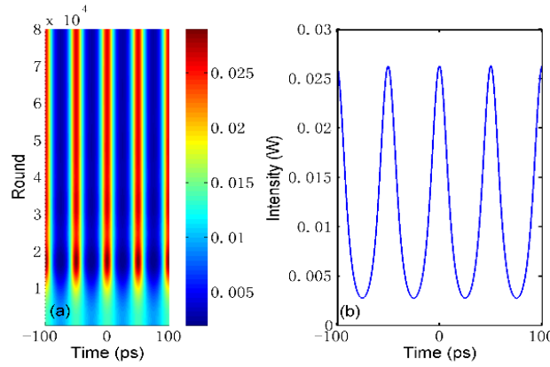
Figure 2.1. (a) Formation of stable periodic pulse pattern in a fiber laser under the effect of modulation instability and effective gain bandwidth limiting. E_s = 0.3\text{pJ} , \Omega_g = 20\text{nm} and f_c = 20\text{GHz} . (b) A steady state laser emission.
