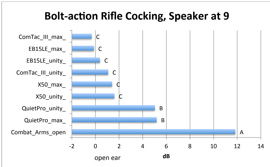
Figure 28. Detection test result for Bolt-action Rifle Cocking from the speaker located at 9 o'clock. X-axis measure is the dB amount by which the performance with the device is worse than the open ear threshold level in dB. (Means with different letters are significantly different at p < 0.10 .) The score computed for each device is the dB difference between threshold level of detection with the device and with the open ear, per the REAT protocol (see text). Thus, for the graph, the open ear score is represented by 0 dB.
