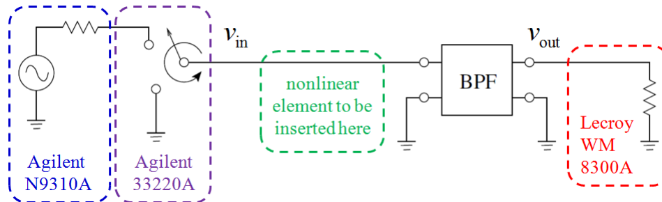
Fig. 1 Switch-and-filter experiment: equipment and arrangement
