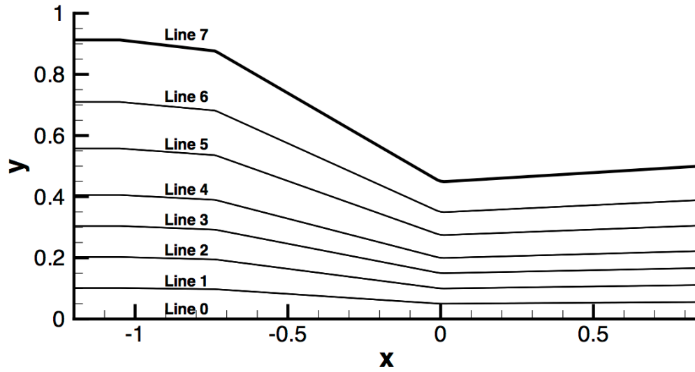
Figure 16. Lines of constant \eta in the physical domain along which computed results are shown.
