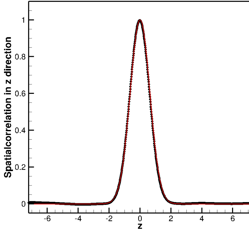
Figure 10. Comparison between input two-point cross correlation function and the computed cross correlation function. Here z = (z' - z'') .
