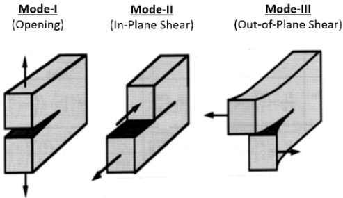
Figure 1. Fracture Modes
