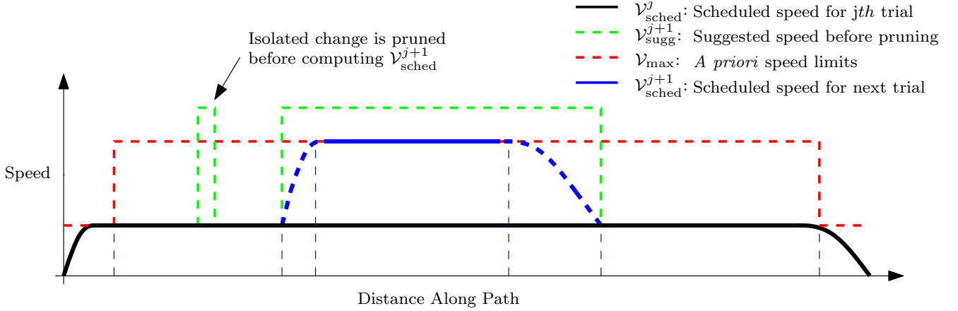
Figure 4. Experience-based speed scheduling occurs in two steps: 1) modifications to the previous speed schedule are suggested based on experience (Green), 2) the suggested speeds are constrained by a priori speed and acceleration constraints (Blue).
