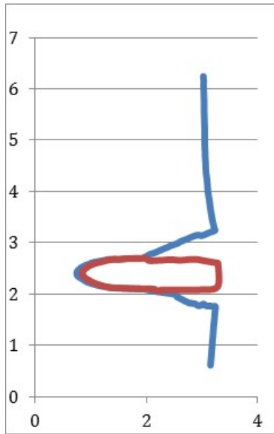
Fig. 8 Dimensionless outline of the penetrator core and target crater from shot no. 12688 with 1.85° of yaw
