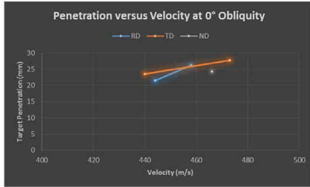
Fig. 6 Initial penetration trends
