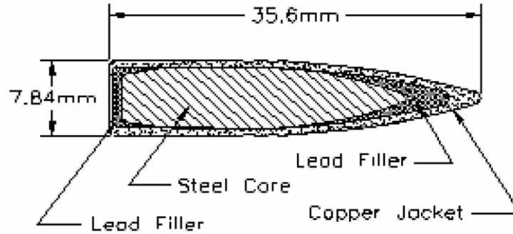
Fig. 2 Sketch of 7.62-mm APM2 projectile
