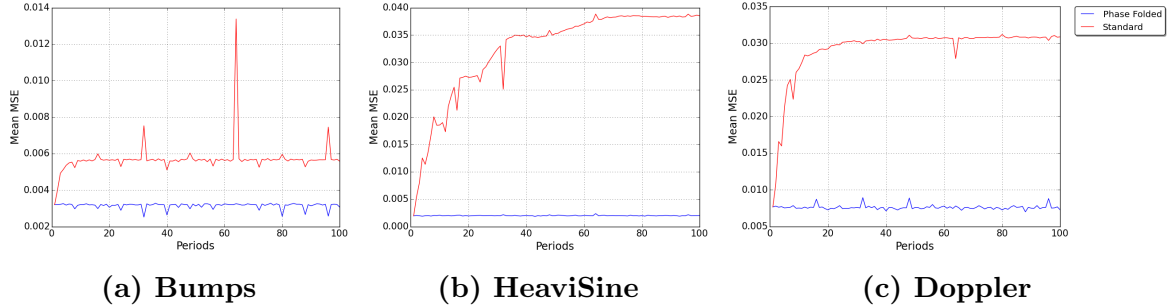
Figure 20. Mean Squared Error for 2^{11} Points with an SNR of 5 dB.
