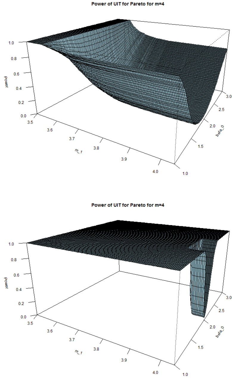
Figure 8. Surface plot of power for the Pareto UIT for k = 5, 10 and m = 4 .
