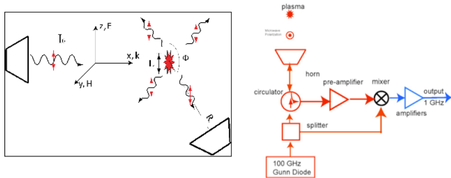
Figure 1: The Radar REMPI coherent homodyne detection process. Left – the laser created ionization region scatters microwave radiation. Right – the microwave scattering is routed to a pre amplifier and mixed with the original microwave source for coherent homodyne detection.
