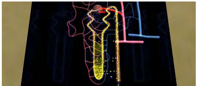
Figure 4 – Virtual Nephron
