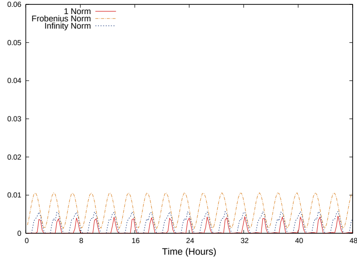
Figure 3.4: Norms of Phi Difference: e = 0.001
