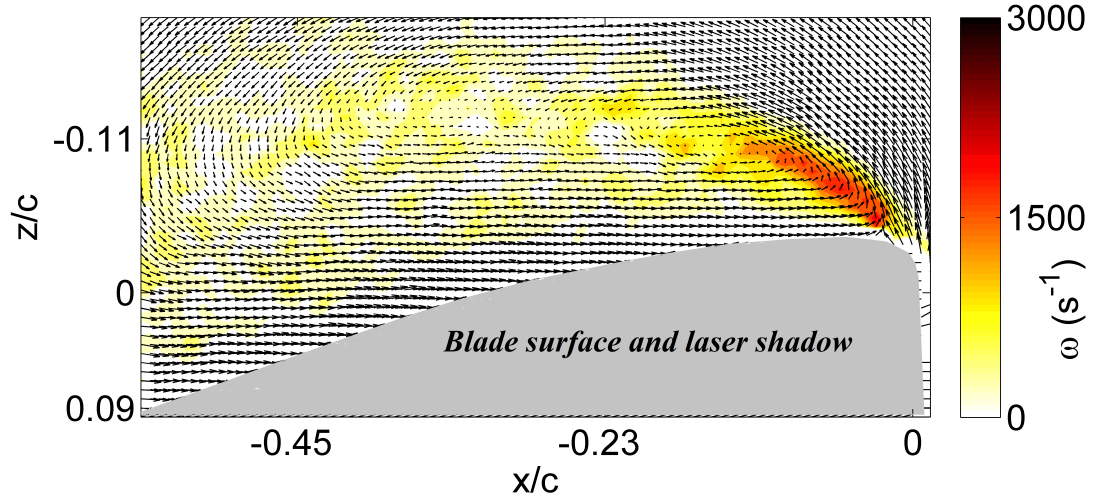
Figure 30: Velocity field at \psi = 270^\circ , r/R = 0.6 , \mu = 0.4
