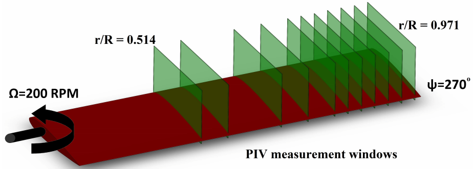
(b) PIV interrogation windows over the radius of the blade
