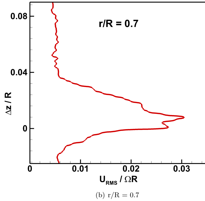
Figure 78: RMS fluctuations showing the peak occurring near the blade surface
