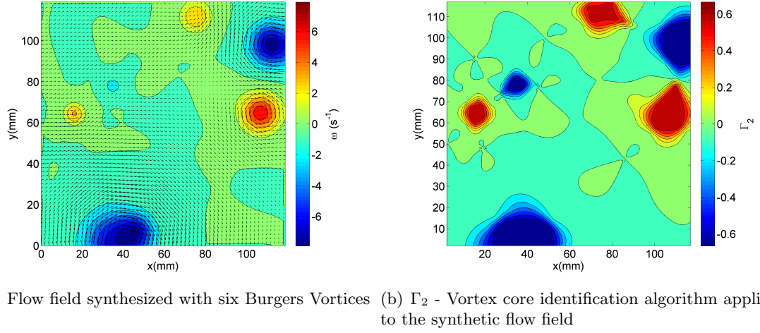
Figure 116: Validation of the vortex core identification technique ( \Gamma_2 )
