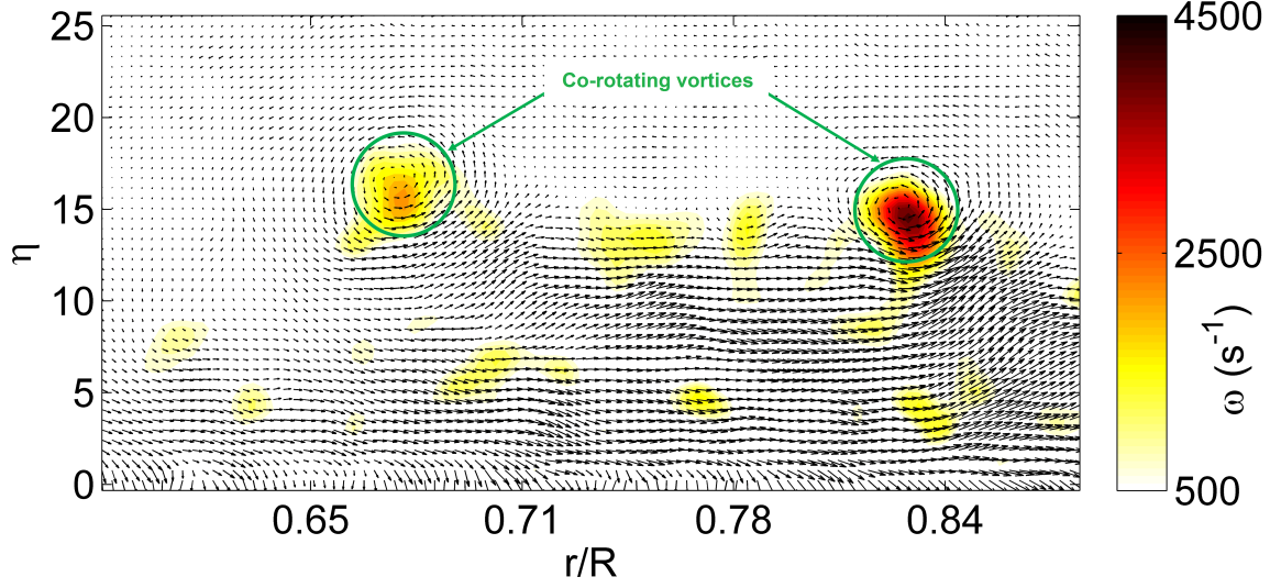
Figure 91: PIV velocity vector field illustrating a typical set of co-rotating vortices above the rotating disk at Re=178 , \mu = 0.69 and \alpha = 8^\circ
