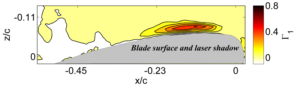
Figure 39: NAM plot at \psi = 315^\circ , r/R = 0.6 , \mu = 0.4
