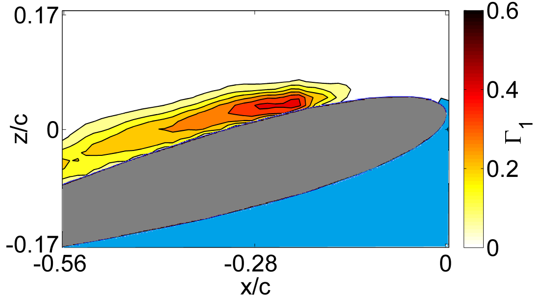
Figure 56: NAM at r/R = 0.743 , k = 0.24 , Re = 87,767
