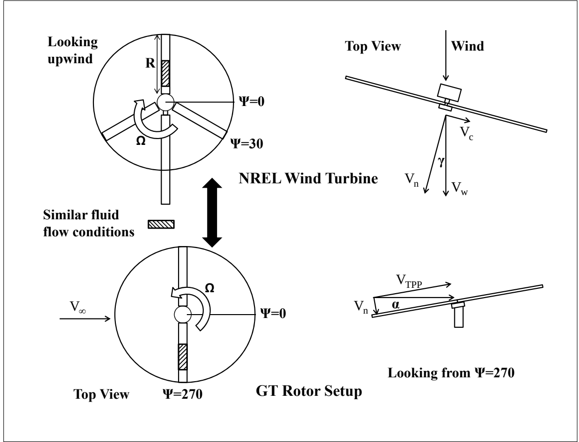
Figure 113: Schematic representation of similar fluid flow conditions.
