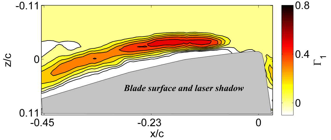
Figure 24: NAM plot at \psi = 235^\circ , r/R = 0.6 , \mu = 0.35
