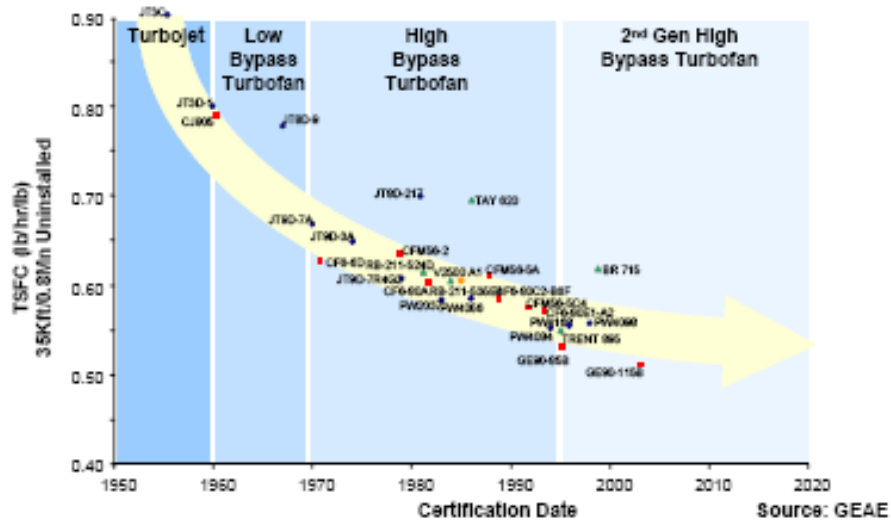
Figure 11: Evolution of Gas-Turbine Fuel Efficiency 46 (Source: GE Aircraft Engines, through Scientific Advisory Board)
