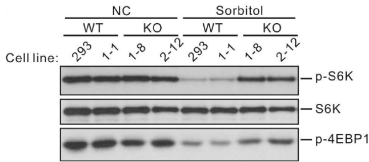
Fig.5. Nlk deletion compromises mTORC1 inhibition upon hyperosmotic stress. WT (293 and 1-
