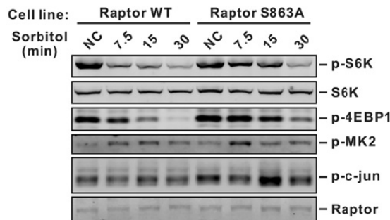
Fig.8. Raptor S863 phosphorylation is important for proper mTORC1 inhibition by osmotic stress. Cells containing WT or S863A Raptor knockin were treated with sorbitol (0.1 M) for the time indicated.
