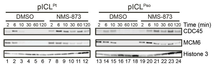
Figure 3: p97 is required for CMG unloading – plasmid pull-down assay. Plasmids containing a cisplatin or psoralen ICL were replicated in the presence DMSO or NMS-873, as indicated. At different times, plasmids were pulled down and the chromatin samples blotted for the indicated antibodies.
