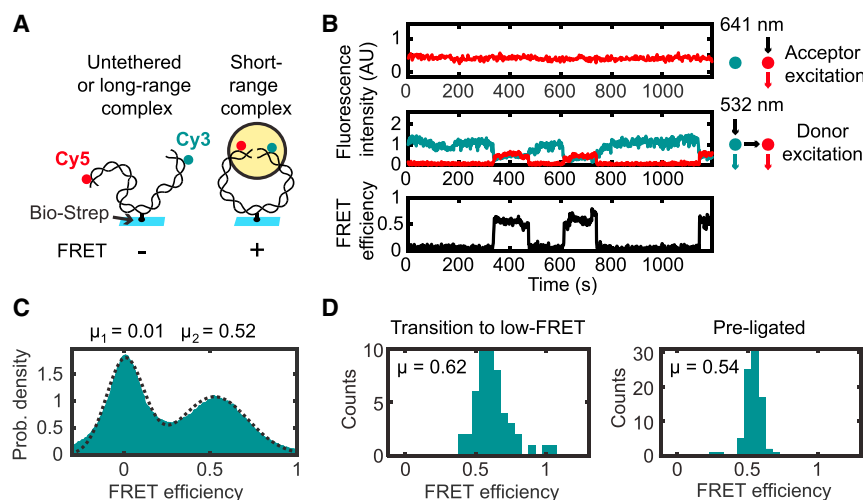
Figure 3. Single-Molecule Circularization Assay
