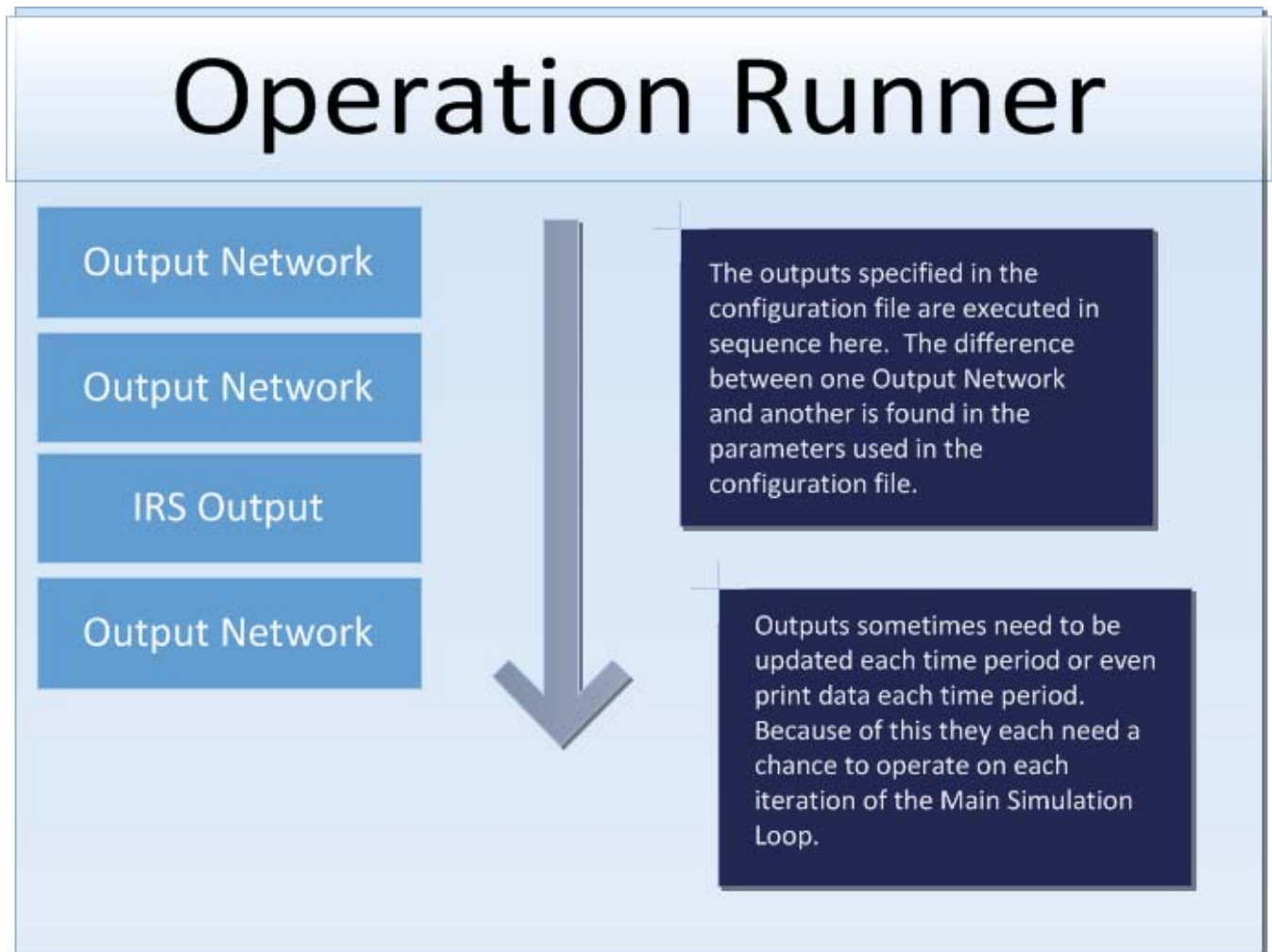
Figure 7. Operation Runner allows for various operations to take place. Operations can be ordered by the user.
