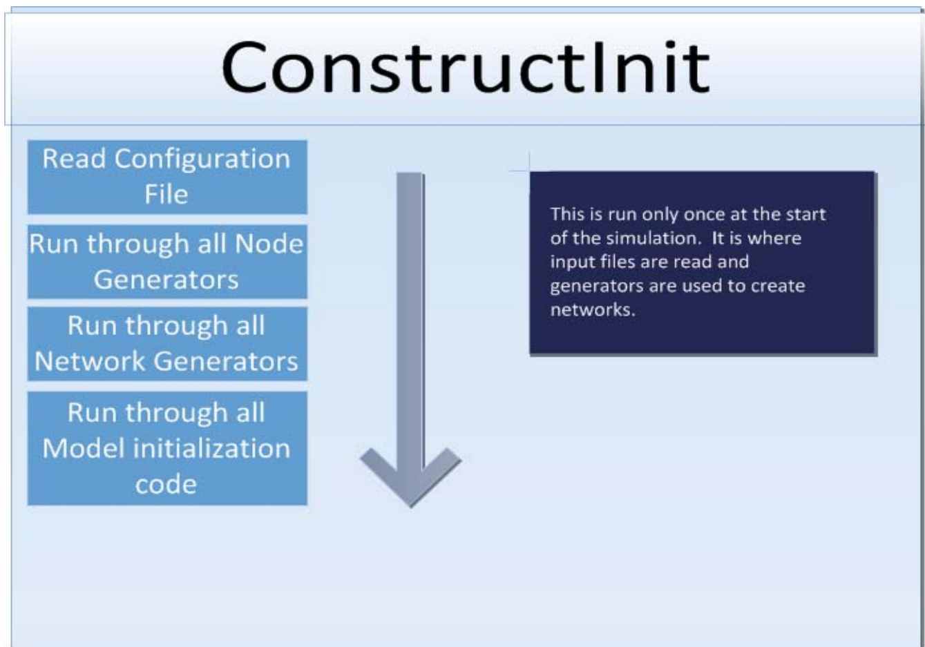
Figure 5. Construct's initialization process starts by reading the deck, then initializes nodes and networks, then goes through model specific setup.
