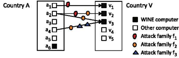
Figure 3: Toy example.
