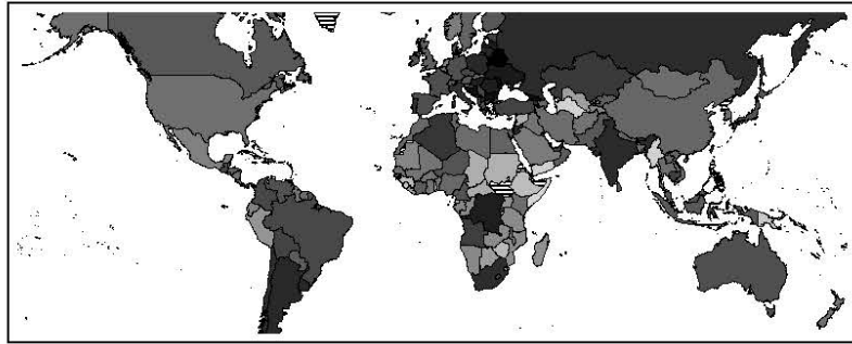
(a) Exploits
