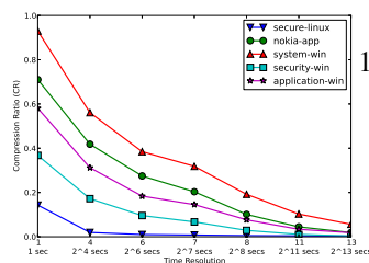
Figure 5: Compression ratio of SF in different resolution
