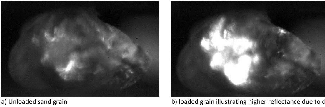
Figure 6. A single grain of sand before and after the crack face has formed. We observe that the presence of the crack results in greater reflectivity and thus more light collected.
