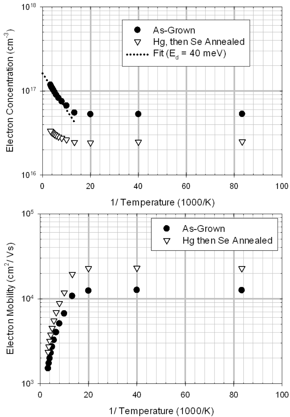
Figure 5-29: Electron concentration (Top) and mobility (Bottom) vs. temperature SZ106 ( x=0.28 ) both as-grown, and after annealing under Hg, then Se for 24 hours each at 250 °C, as well as a fit to concentration at higher temperatures.
