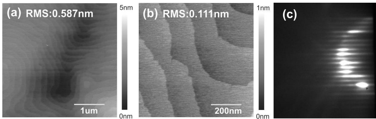
Figure 4-11: Images of homoepitaxial GaSb (100) (Sample 7-166) taken by AFM (a), (b) and RHEED (c).
