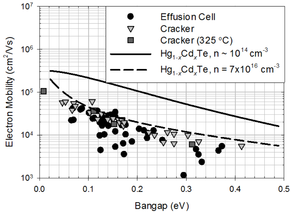
Figure 5-13: As-grown electron mobility vs. energy bandgap at 77K for \text{Hg}_{1-x}\text{Cd}_x\text{Se} samples grown with the effusion cell ( 5\text{N} \sim \text{Se}_6 ), the cracker ( 6\text{N} \sim \text{Se}_2 ) and the cracker with the cracking zone lowered to 325^\circ\text{C} ( 6\text{N} \sim \text{Se}_6 ). Also included is the predicted 77K \text{Hg}_{1-x}\text{Cd}_x\text{Te} mobility for both low doping ( n \sim 10^{14} \text{ cm}^{-3} ), and for n = 7 \times 10^{16} \text{ cm}^{-3} , N_i = 1.7 \times 10^{17} \text{ cm}^{-3} .
