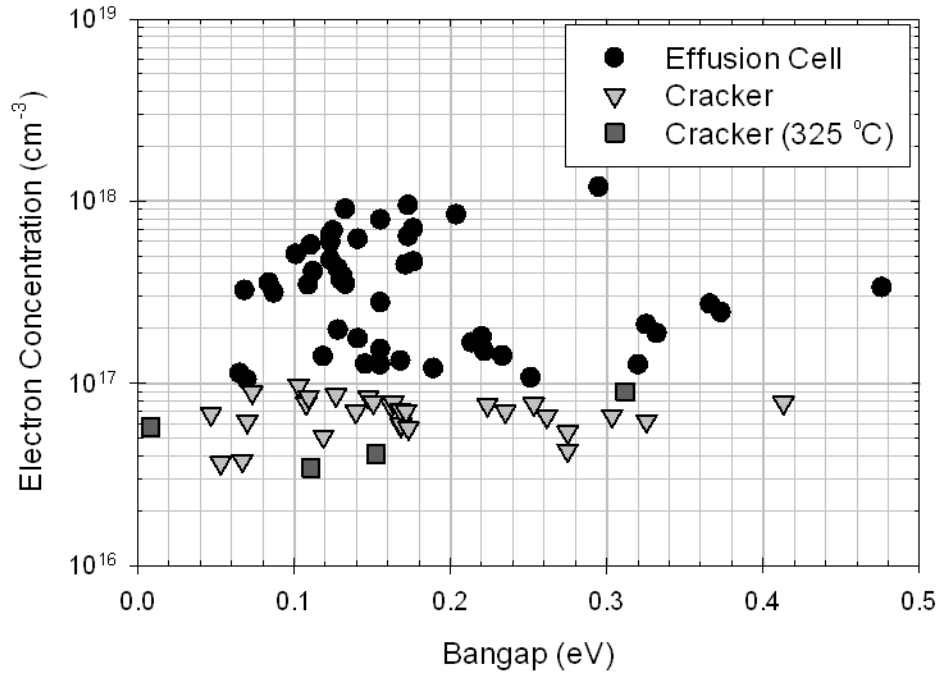
Figure 5-12: As-grown electron concentration vs. energy bandgap at 77K for \text{Hg}_{1-x}\text{Cd}_x\text{Se} samples grown with the effusion cell ( 5\text{N} \sim \text{Se}_6 ), the cracker ( 6\text{N} \sim \text{Se}_2 ) and the cracker with the cracking zone lowered to 325^\circ\text{C} ( 6\text{N} \sim \text{Se}_6 ).
