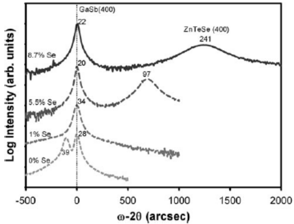
Figure 4-18: XRD scans of \text{ZnTe}_{1-x}\text{Se}_x layers grown on GaSb for several Se compositions. Numbers indicate the FWHM of each peak. The angle of the GaSb peak was set to zero.
