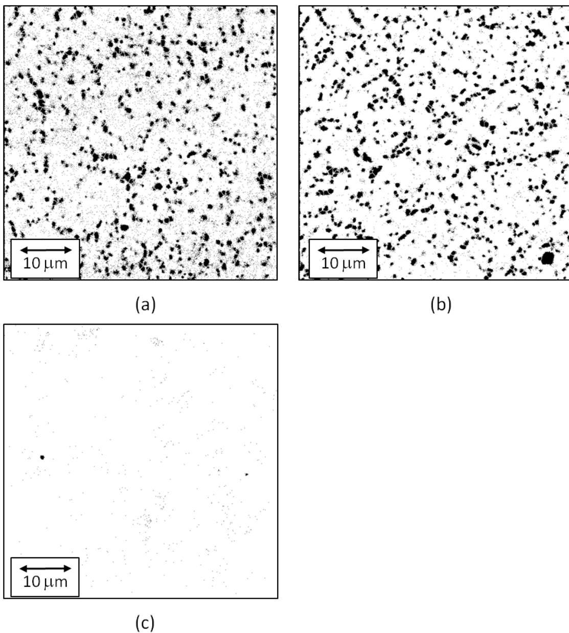
Figure 4-20: cPL images of (a) Z49, 2 μm-thick ZnTe/GaSb (211)B; (b) Z140, 2 μm-thick ZnTe/GaSb (100); and (c) Z74, 1.2 μm-thick \text{ZnTe}_{0.99}\text{Se}_{0.01} /GaSb (211)B. Each image represents an area of 54 μm x 54 μm.
