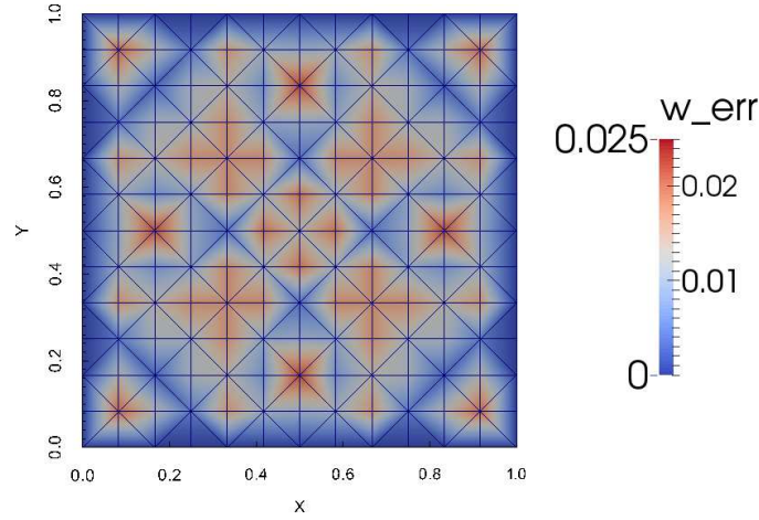
Figure 1.2: Deformation error of a square membrane subjected to uniform pressure.
