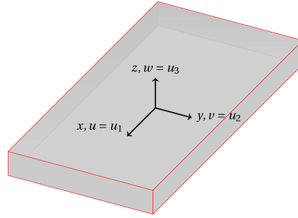
Figure 1.1: Membrane model.
