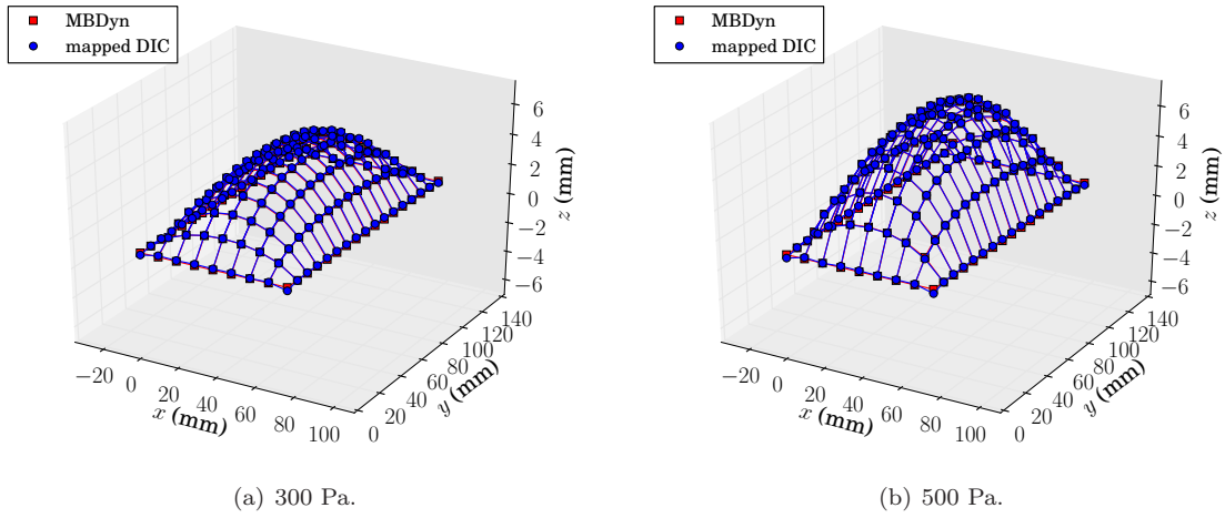
Figure 2.3: Numerical/experimental correlation of hydrostatic pressure problem.
