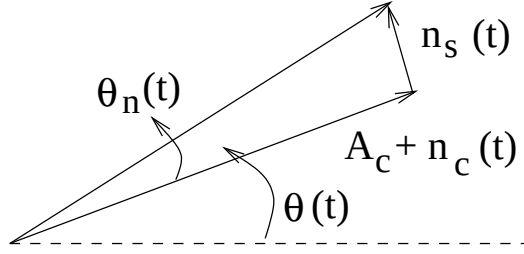
Figure 5.34: I and Q components of a noisy angle modulated signal with the phase reference chosen as the phase of the noiseless signal.
