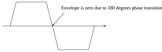
Figure 4.20: The envelope of a PSK signal passes through zero during a 180 degree phase transition, and gets distorted over a nonlinear channel.
