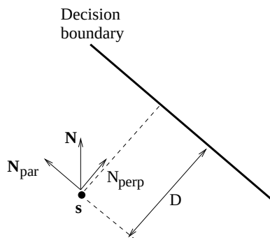
Figure 6.17: Only the component of noise perpendicular to the decision boundary, N_{\text{perp}} , can cause the received vector to cross the decision boundary, starting from the signal point \mathbf{s} .
