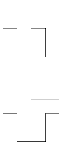
Figure 4.16: Walsh-Hadamard codes for 4-ary orthogonal modulation.
