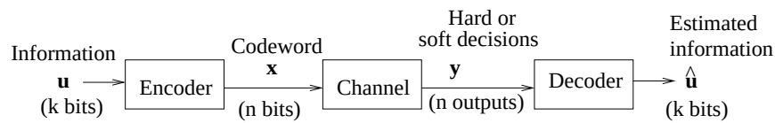
Figure 7.3: High-level model for coded system.
