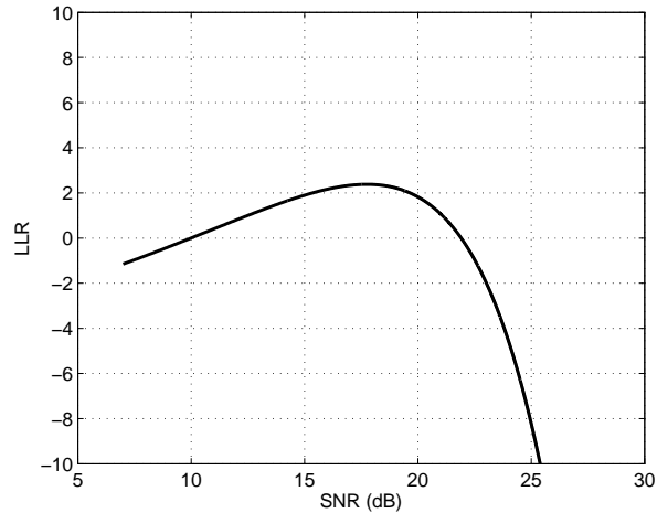
Figure 4. LLR for K-distribution clutter
