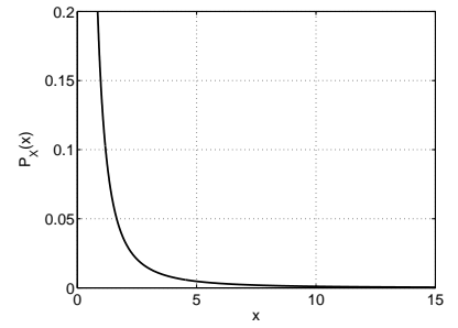
Figure 7. PDF of X for \alpha_k = 5
