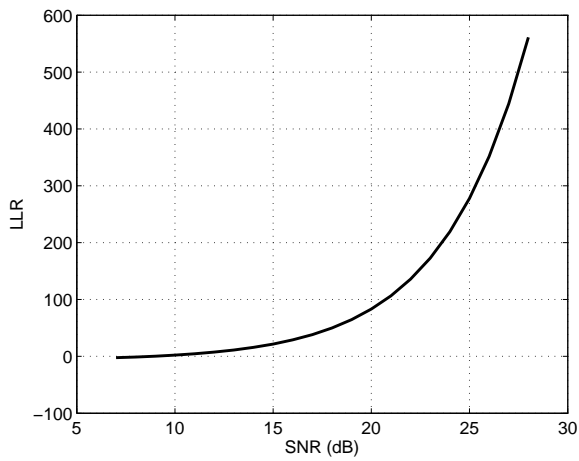
Figure 3. LLR for Rayleigh distribution clutter
