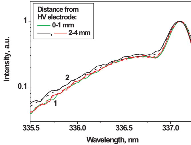
Figure 4.10: Rotational structure of second positive system of nitrogen in synthetic air. The spectra are taken for P = 3 bar: (1) quasi-uniform mode, U_1 = -36 kV; (2) filamentous mode, U_3 = -55 kV. For the quasi-uniform mode, the emission is collected from different distances from the edge of HV electrode, as indicated in the figure. Dashed lines correspond to theoretical approximations at the given temperature (see text).
