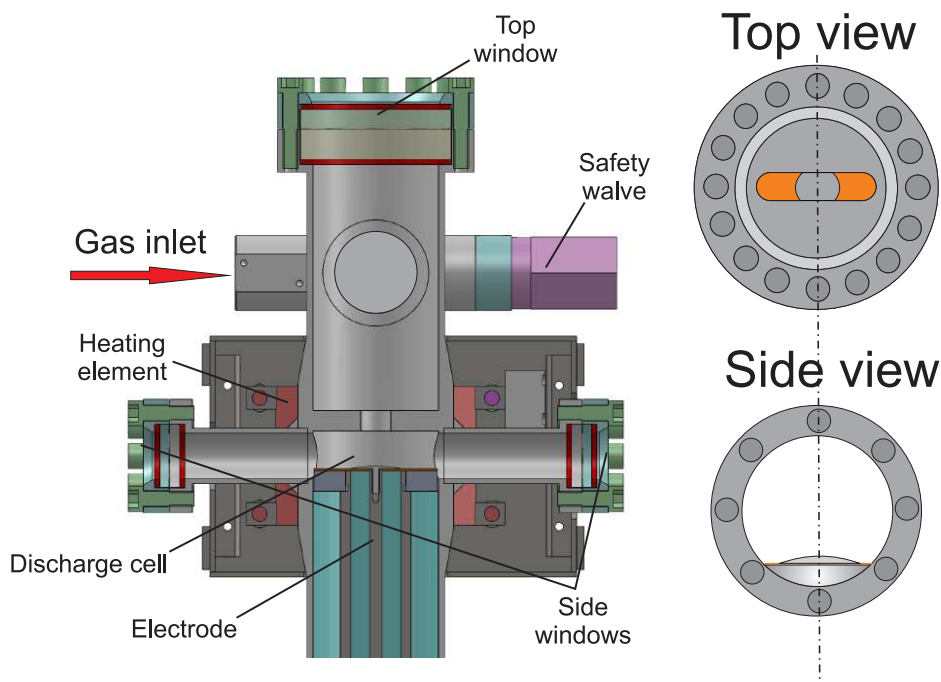
Figure 7.2: The schematic representation of High-Pressure High-Temperature (HPHT) reactor and the views of the flanges (top, side).
