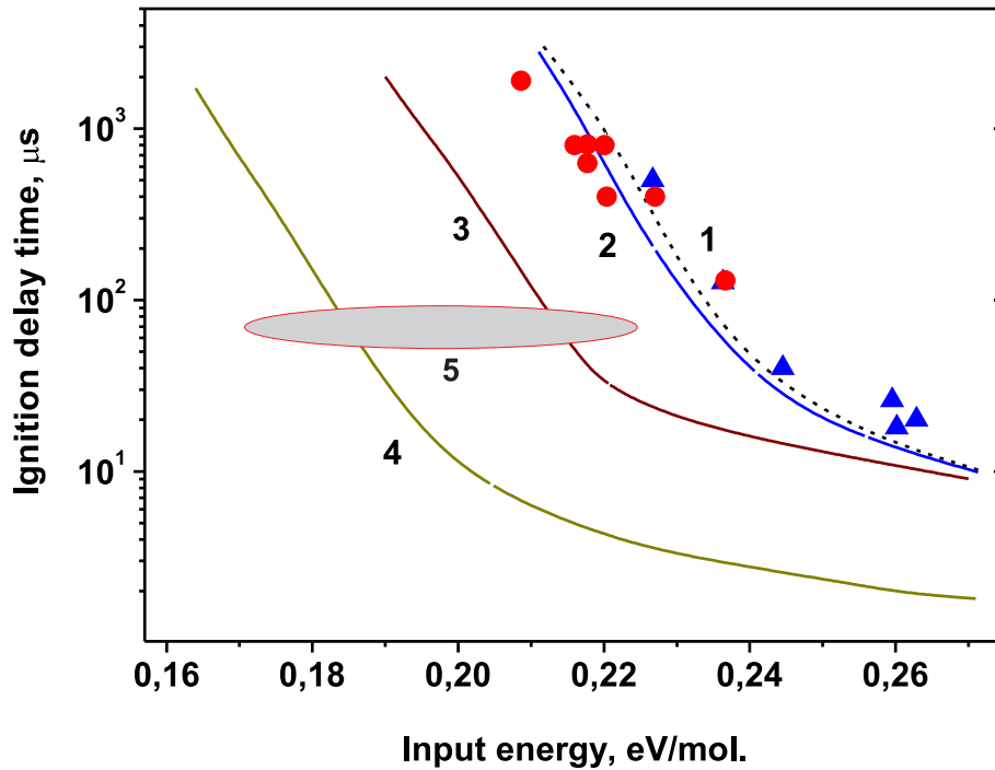
Figure 7.16: The induction delay time as a function of specific energy. \text{H}_2/\text{air} mixture, P=4\text{--}6 bar, T_0=300 K, ER=0.44\text{--}0.5 . Results of simulation (curves 1,2) and experimental data (dots) [44], for the conditions when the total energy of the discharge instantly goes to the gas heating; ER = 0.44 , P = 4 bar (curve 1), P = 6 bar (curve 2). Curves 3 and 4 correspond to the simulation with real energy distribution over the degrees of freedom at E/N = 100 Td (3) and E/N = 200 Td (4), ER=0.5 , P=6 bar. The shaded area 5 is the experimental data on the induction delay time \tau_{ind}=50\text{--}70 \mu\text{s} , obtained in given work.
