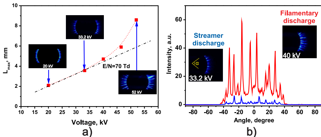
Figure 7.8: (a) Maximal length of discharge propagation in H_2 :air mixture as a function of applied voltage. P = 6 bar, T = 300 K, ER = 0.5 ; (b) comparison of angular distribution of emission intensity for streamers, U = +33 kV and filaments, U = +40 kV on the high-voltage electrode.
