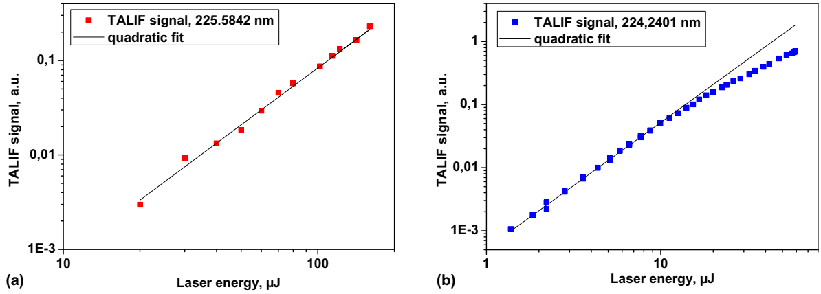
Figure 2.10: Calibration curves for (a) oxygen atoms, 27 mbar synthetic air, 2500 K, 2.2 \mu s after breakdown and (b) xenon atoms, 8.6 mbar pure xenon, 293 K, no discharge.
