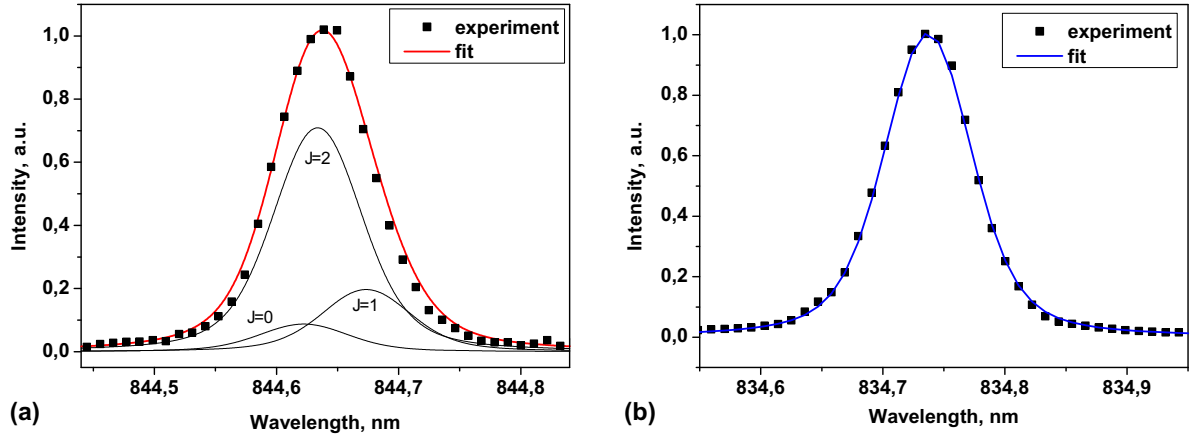
Figure 2.9: TALIF dispersed fluorescence signal taken with a spectrograph and ICCD camera. (a) oxygen atoms, laser wavelength 225.583 nm, 27 mbar synthetic air, 2500 K, 2.2 \mu s delay after first discharge; (b) xenon atoms, laser wavelength 224.238 nm, 8.6 mbar pure xenon, 293 K, no discharge.
