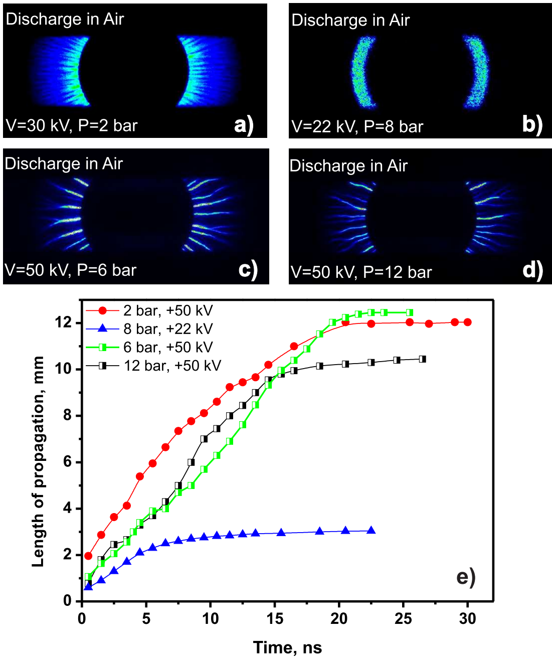
Figure 7.6: Integral ICCD images of positive polarity nanosecond surface barrier discharge (nSDBD) in air for different voltage of applied pulses and pressures: (a) U = +30 kV, P = 2 bar, (b) U = +22 kV, P = 8 bar, (c) U = +50 kV, P = 6 bar, (d) U = +50 kV, P = 12 bar. ICCD camera gate is 100 ns, pressure and voltage are indicated at each frame. (e) Selected x-t diagrams. ICCD gate is 0.5 ns.
