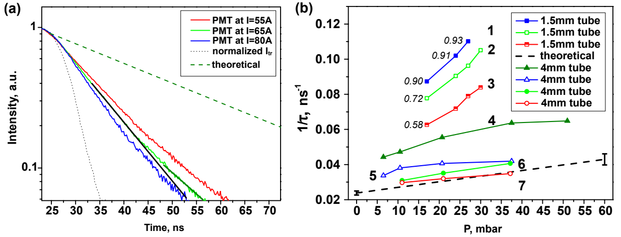
Figure 3.3: Experimental results for \text{N}_2(\text{C}^3\Pi_u, v' = 0) quenching in a capillary tube in pure nitrogen: (a) experimentally measured emission at 27 mbar for different discharge current; dashed line represents nitrogen emission calculated on the basis of quenching by \text{N}_2 with rate constant from [18]; dot line shows a normalized waveform for electric current; (b) reverse decay time \tau_1 as a function of pressure for different specific deposited energies. Specific deposited energy decreases with the number of curve, see detailed explanations in the text. Dashed curve is for theoretical prediction.
