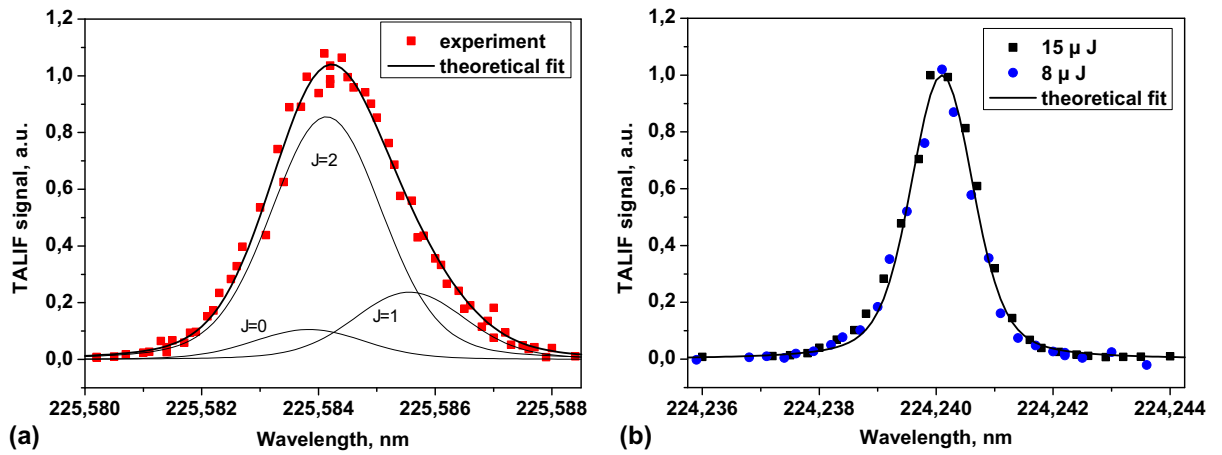
Figure 2.8: TALIF PMT signal integrated in time, plotted as a function of laser wavelength. (a) O atoms, 27 mbar synthetic air, 2500 K, 2.2 \mu s after breakdown, laser energy 108 \mu J; (b) Xe atoms, 8.6 mbar pure xenon, 293 K, no breakdown, laser energy 15 and 8 \mu J. The same scale in laser wavelength was used. Note the broad linewidth of the O line, due to the three fine-structure levels of O( 3p^3P ), and the broadening due both to the high temperature of the gas 2 \mu s after breakdown, and the lighter nature of O atoms compared to xenon atoms.
