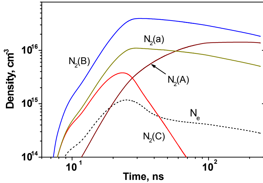
Figure 3.6: Kinetic curves of the main exited species of the molecular nitrogen at the axis of the discharge tube calculated for the first pulse coming to the capillary tube at the same conditions as for figure 3.5.
