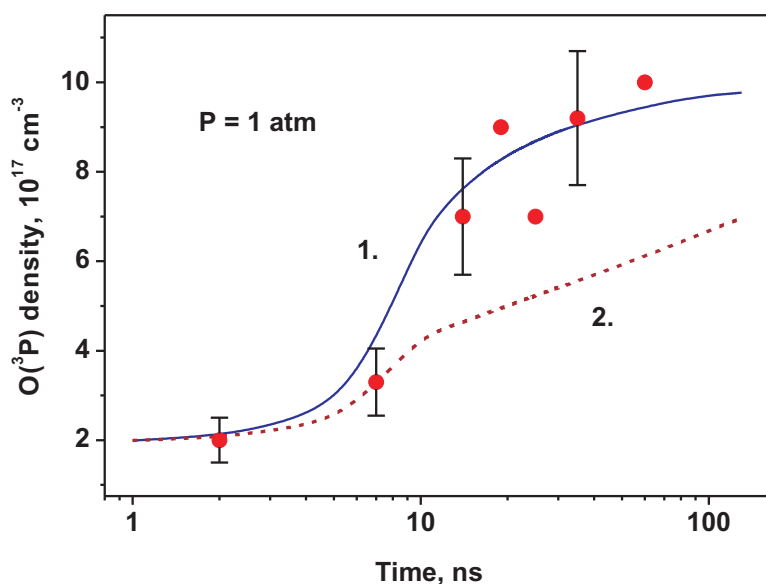
Figure 9.2: Time evolution of the density of \text{O}(^3\text{P}) atoms under the conditions of [16, 17]. The dots are for the experimental data from [16], and the curves 1 and 2 are for the numerical results [18] at the discharge axis (see text).
