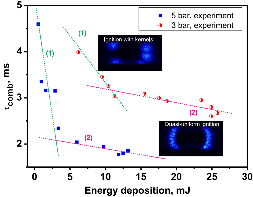
Figure 7.14: Time of initiation of combustion in entire volume as a function of delivered energy for different pressures. H 2 :air mixture, ER = 0.6 .
