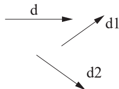
Figure 6: direction \vec{d} is between (\vec{d}_1, \vec{d}_2)
