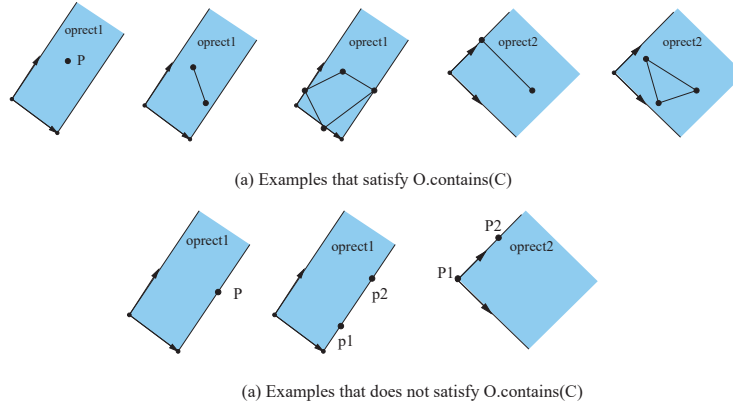
Figure 24: Examples of contains relationship
