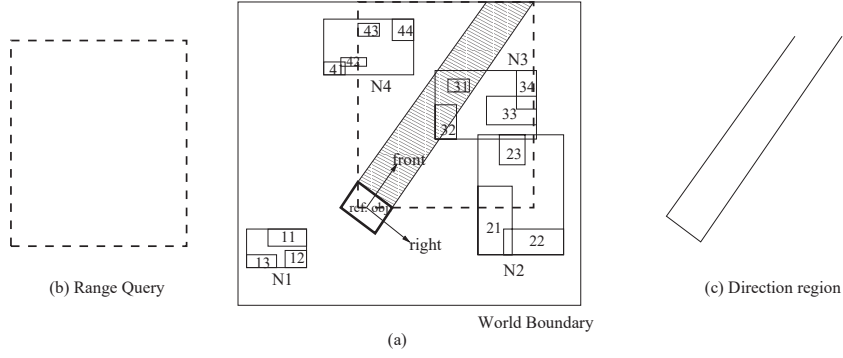
Figure 5: Processing object-orientation-based query using range query strategy
