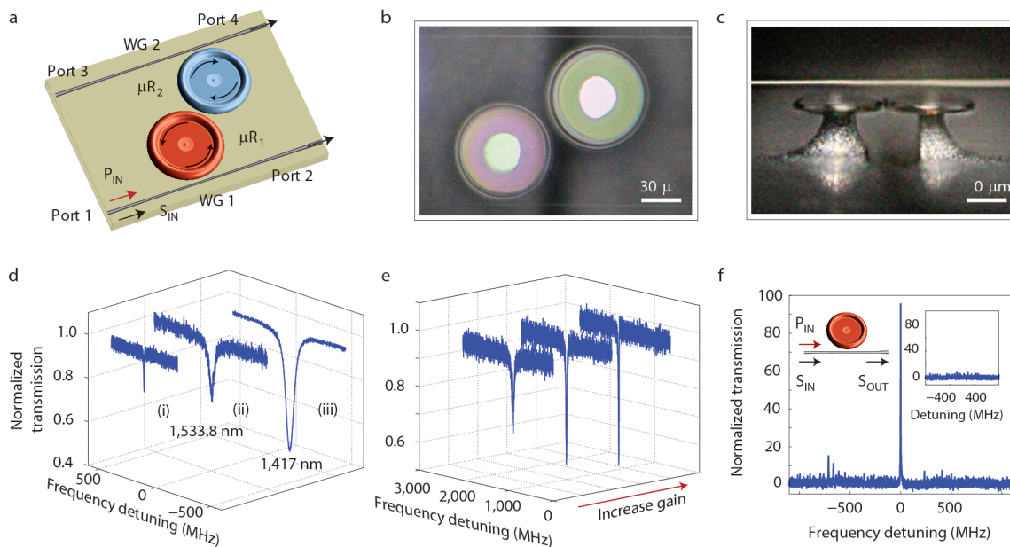
Figure 1 | PT-symmetric whispering-gallery-mode microcavities. a , A system consists of two directly coupled whispering-gallery-mode resonators (W GMRs) and two fibre-taper waveguides. WG1: fibre-taper waveguide with ports 1 and 2. WG2: fibre-taper waveguide with ports 3 and 4. \mu R_1 : active \text{Er}^{3+} -doped silica microtoroid. \mu R_2 : passive silica microtoroid. P_{\text{IN}} : pump laser in 1460 nm band to excite \text{Er}^{3+} ions that provide gain in 1,550 nm band. S_{\text{IN}} : probe light (signal) in 1,550 nm band. b, c , Top and side views of the coupled resonators. d , Transmission spectra showing resonance of \mu R_2 at 1,533.8 nm (i) and resonances of \mu R_1 at 1,533.8 nm (ii) and at 1,417.0 nm (iii). e , Gain provided by \text{Er}^{3+} ions in \mu R_1 leads to narrower and deeper resonances as pump power (gain) is raised, implying an increasing Q-factor. f , Weak probe light is amplified when coupled to \mu R_1 together with the pump light. Inset shows that without the weak S_{\text{IN}} there is no resonance enhancement.
