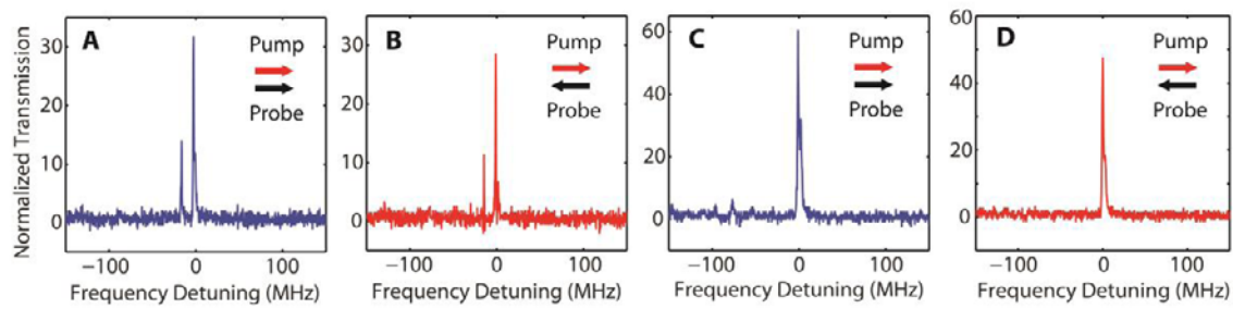
Fig.S8. Experimentally obtained transmission spectra in broken- and unbroken-PT-symmetric regions with different pump and probe directions. In these experiments the configurations in Fig. S4A are used. (A) and (B) are obtained in the unbroken-symmetry region using Fig. S4A(i) and Fig. S4A(ii), respectively. (C) and (D) are obtained in the broken-symmetry region using Fig. S4A(i) and Fig. S4A(ii), respectively. The transmission spectra are the same regardless of the directions of the pump and probe light fields.
