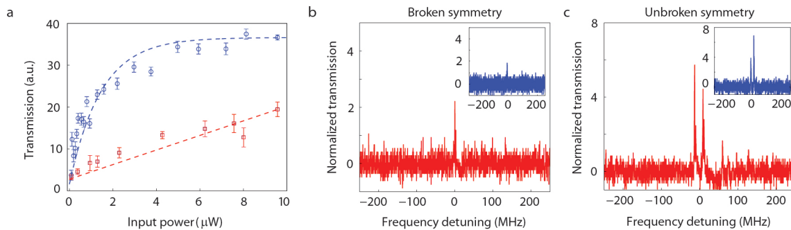
Figure 3 | Input-output relation in PT-symmetric WGMRs and reciprocity in the linear regime. a , Linear input-output relation in the unbroken-symmetry region (red square symbols) but nonlinear in the broken-symmetry region (blue circle symbols). Transmitted signal to port 1 was detected by a photodetector when the input was at port 4. Each data point is the average of ten measurements, and the error bars represent the standard deviations. b, c , Transmission spectra in the linear regime (input power of 80 nW) show reciprocal light transmission at forward (blue inset) and backward (red spectra) directions in both the broken- ( b ) and unbroken- ( c ) symmetry regions. The red (blue) spectra were normalized with the signal detected at port 3 (2) when the input was at port 4 (1) and there was no coupling between the fibre tapers and the resonators. The slight difference in the heights of the resonance peaks is attributed to the laser power fluctuations during frequency scanning and to the thermal fluctuations of the environment. These can be minimized, if not completely eliminated, by active stabilization and better control of the experimental conditions (Supplementary Section B10 and Fig. 12).
