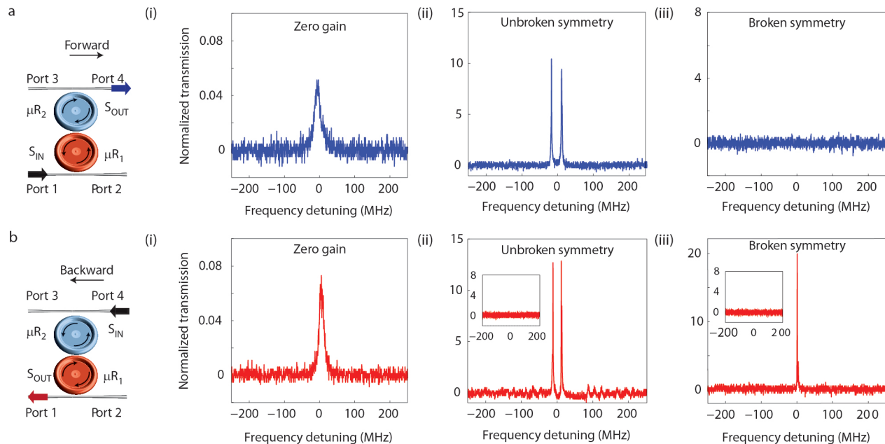
Figure 4 | Experimentally observed unidirectional transmission for PT-symmetric WG M microresonators in the nonlinear regime. a, b , When both resonators are passive (zero gain), the transmission is bi-directional (reciprocal), and light is transmitted in both forward ( a (i)) and backward directions ( b (i)). In the unbroken-symmetry region, where the coupling exceeds the critical value and gain and loss are balanced, the transmission is still bi-directional ( a (ii), b (ii)). Mode splitting due to coupling is now resolved because gain compensates loss leading to narrower linewidths. In the broken-symmetry region ( a (iii), b (iii)), transmission becomes unidirectional (non-reciprocal). Input in the backward direction reaches the output ( b (iii)), but input in the forward direction does not ( a (iii)). This resembles the action of a diode and implies that an all-optical on-chip diode with PT-symmetric WG M microcavities operates in the broken-symmetry region. Inset in ( b (ii), b (iii)) shows the signal at port 1 when there is no input signal at port 4.
