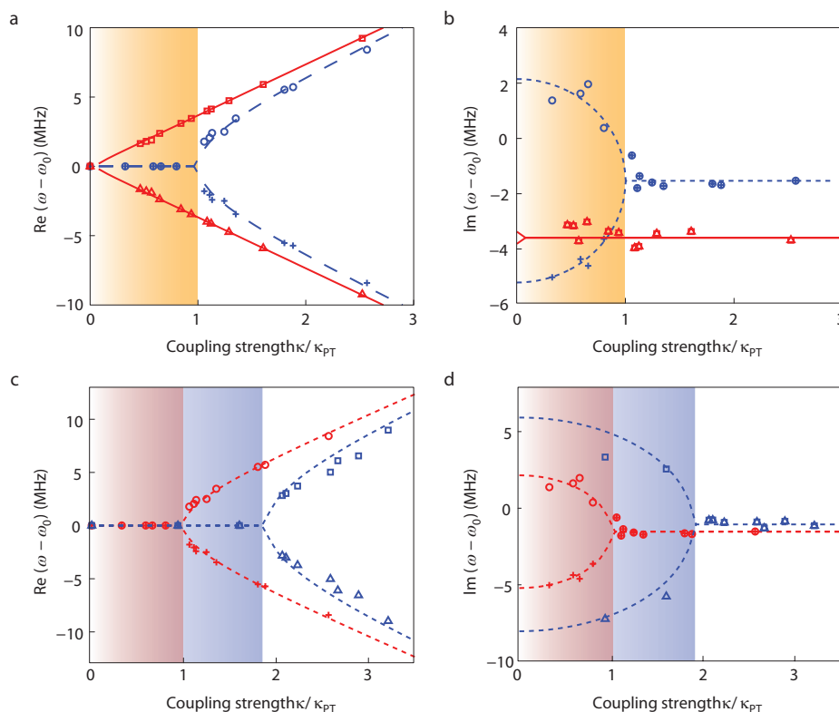
Figure 2 | PT-symmetry breaking in coupled WG M microresonators. a–d , Experimentally obtained real \text{Re}(\omega) ( a,c ) and imaginary \text{Im}(\omega) ( b,d ) parts of the eigenfrequencies of supermodes as a function of coupling \kappa/\kappa_{PT} (Supplementary Sections B2 and B3 and Supplementary Fig. 6). \omega_0 is the frequency of the resonances before coupling. The data points are obtained from curve-fitting the measured transmission spectra to the analytical model. a,b , Comparison when resonators are passive (no gain in \mu R_1 : red square and triangular symbols) with Q-factors 2.9 \times 10^7 and 3.0 \times 10^7 , respectively, for \mu R_1 and \mu R_2 , and when one resonator is active and the other is passive (gain in \mu R_1 : blue circular and cross symbols). c,d , Effect of initial Q-factor (loss) of \mu R_2 on eigenfrequencies. Two resonances with Q-factors 2.0 \times 10^7 (blue) and 3.0 \times 10^7 (red) are chosen for \mu R_2 . Shaded regions correspond to the broken-PT-symmetric region when gain and loss are balanced. The dashed and solid lines were obtained from the theoretical model using experimentally obtained values of coupling strength, gain and the loss parameters (Supplementary Sections B2–B4 and Figs 5 and 6). The value of \kappa_{PT} in c,d is obtained for the case when high Q = 3.0 \times 10^7 resonance mode is chosen in \mu R_2 .
